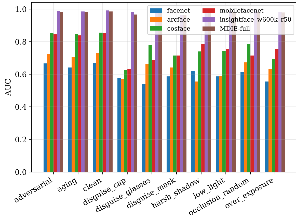
AUC per modification — baselines vs MDIE
