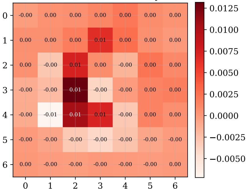
facenet — occlusion sensitivity ( \Delta_{\text{sim}} )
