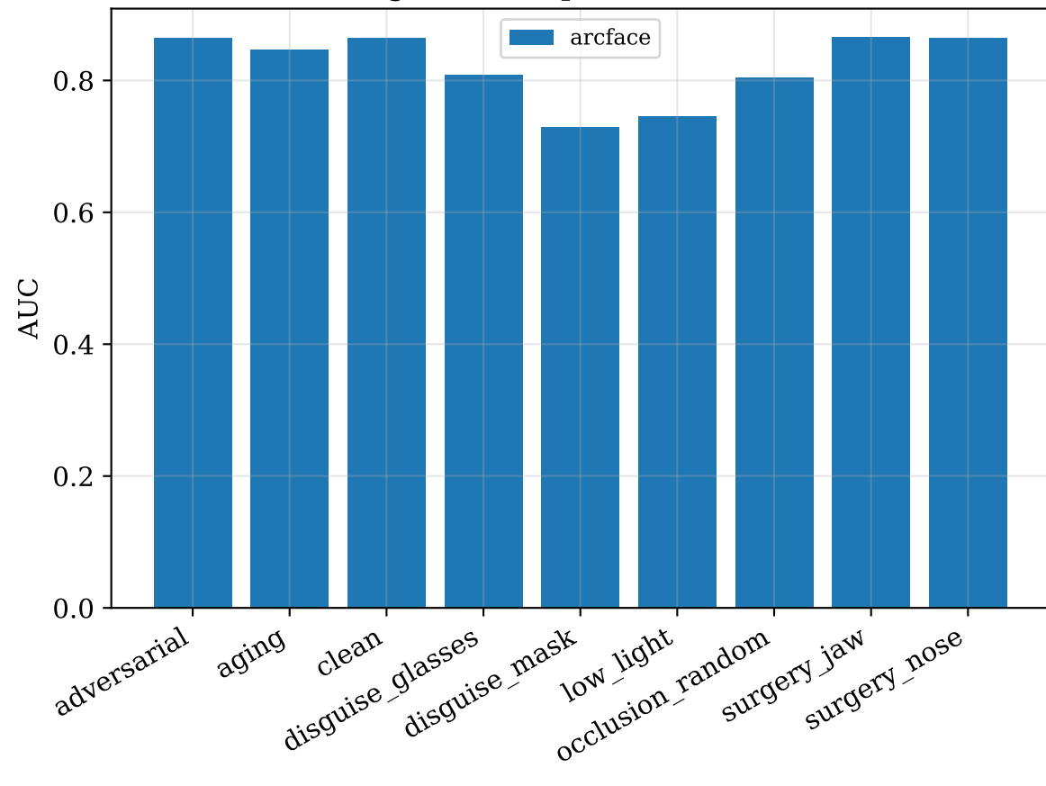
Stage 1: AUC per modification
