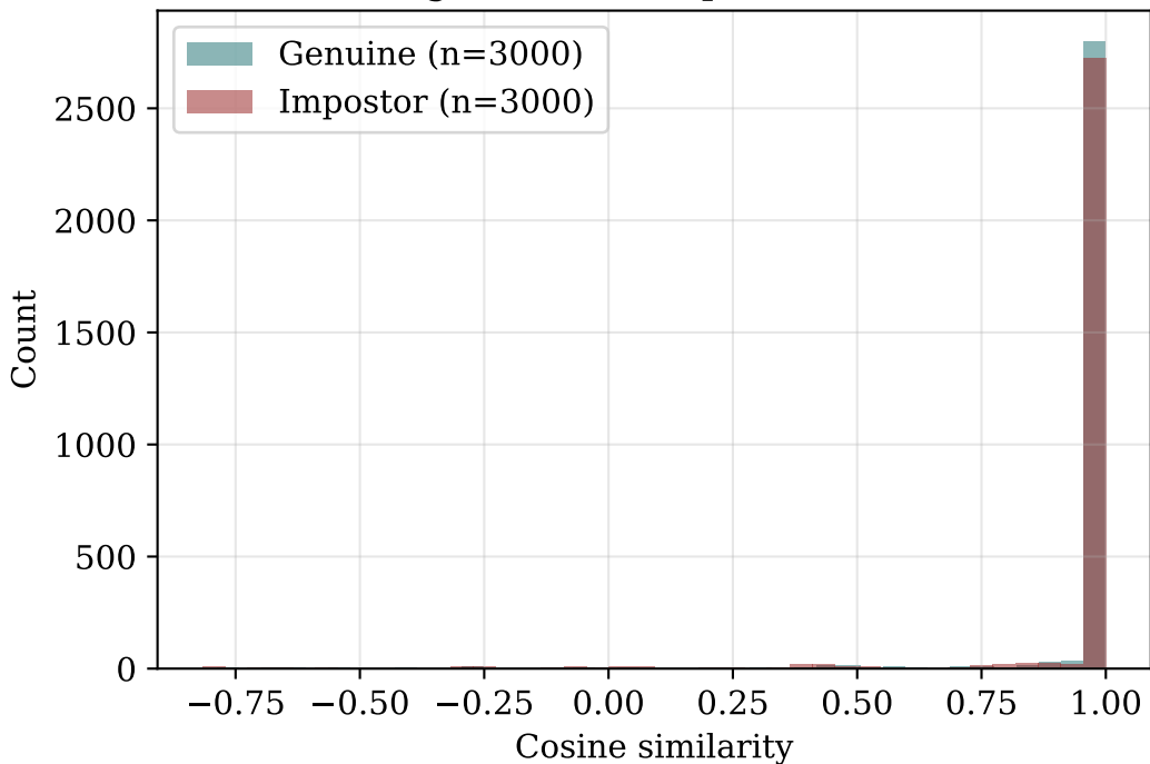
facenet — genuine vs impostor distributions
