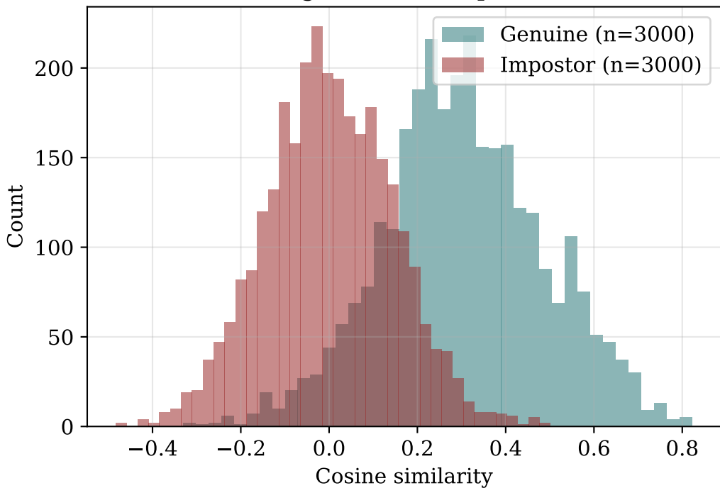
mobilefacenet — genuine vs impostor distributions
