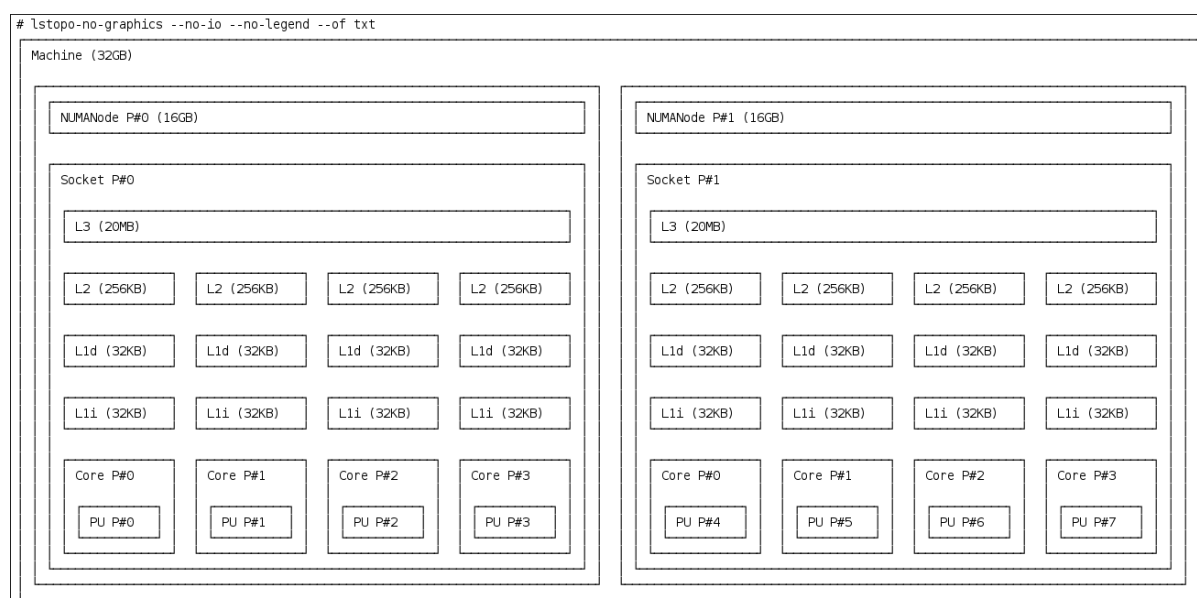
Figure 26.1. Showing the layout of CPUs using lstopo-no-graphics
