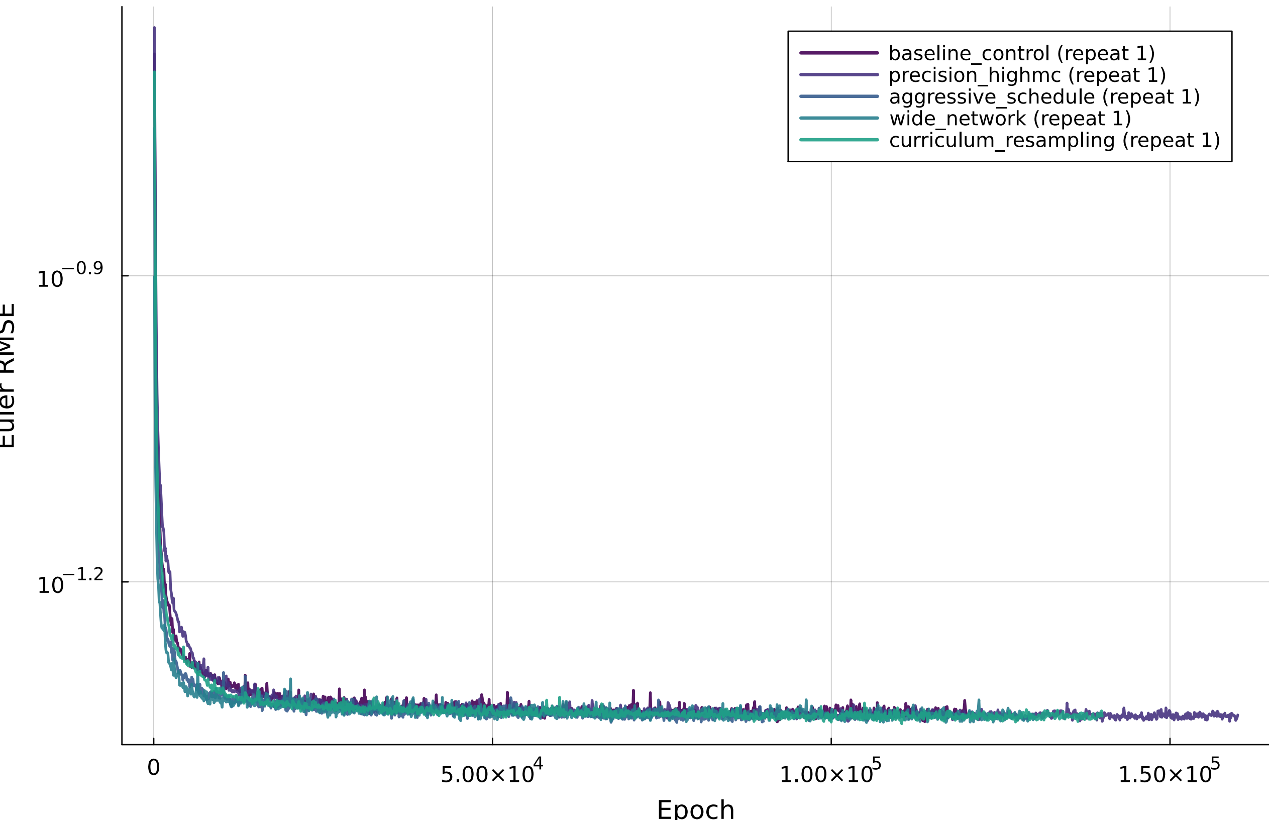
Euler RMSE Trajectories
