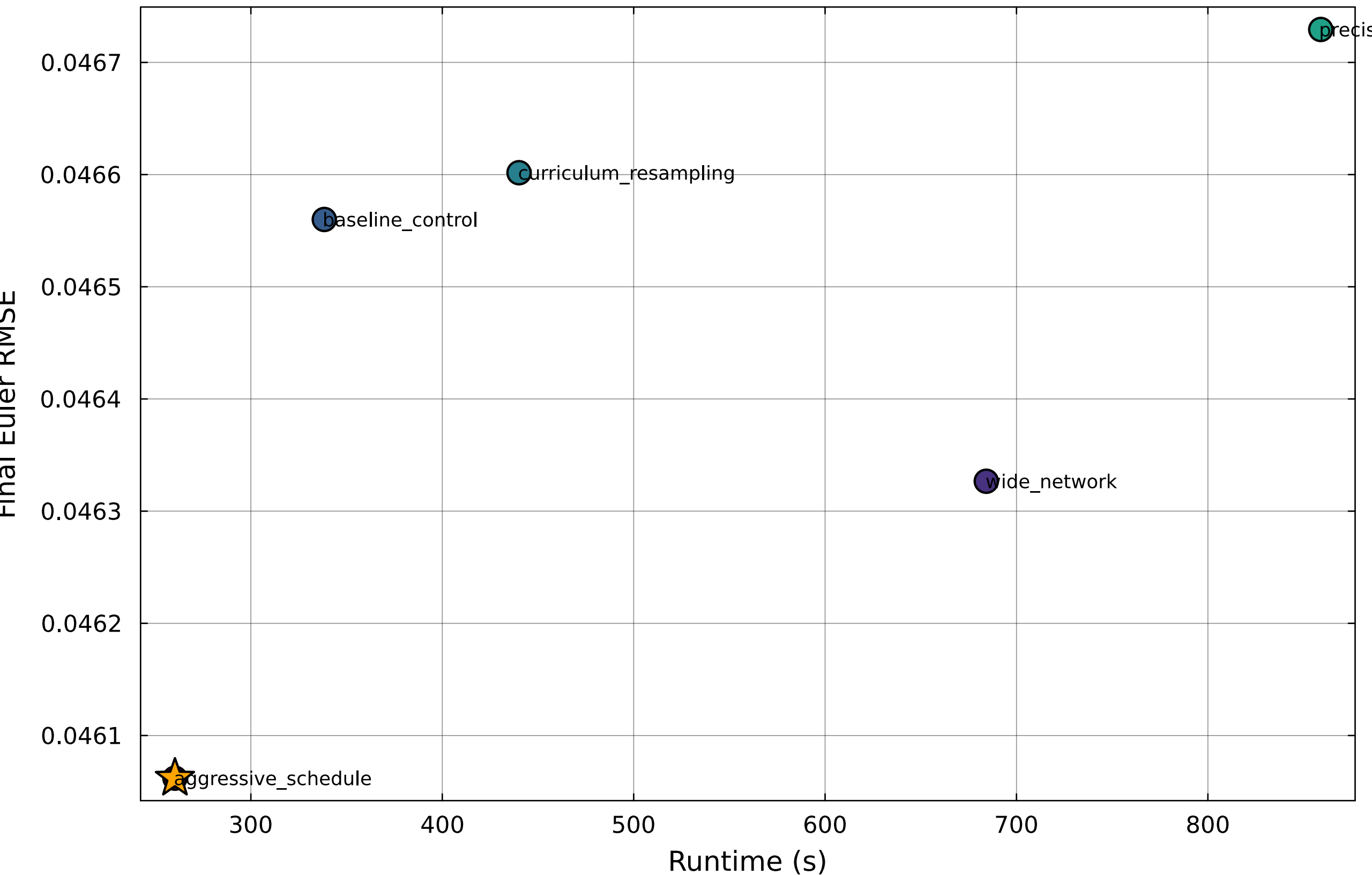
Runtime-Accuracy Frontier
