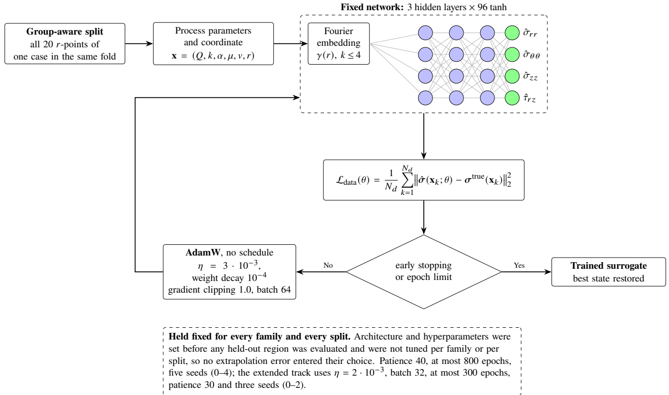
Fig. 2 Training of the data-driven MLP surrogate. The architecture and every hyperparameter are fixed before any held-out region is evaluated. The loop shown is the training loop of a single run, and no hyperparameter search surrounds it.
