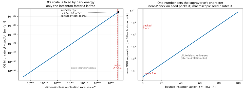
Figure 5.6: Pinning the OG birth rate. Left : \beta = \lambda H_\Lambda^4/c^3 ; the prefactor ( \sim 4 \times 10^{-97} \text{ m}^{-3}\text{s}^{-1} ) is fixed by the observed dark energy, leaving only the instanton factor \lambda = e^{-I} free. Right : the mean OGU separation versus the instanton action I ; the de Sitter percolation threshold I_{\text{crit}} \simeq 1.4 splits a packed polygonal foam (near-Planckian seed) from a dilute scatter of island universes (macroscopic seed). Reproducible as figures/scripts/ch05_birthrate.py.
