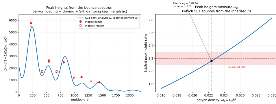
Figure 9.10: CMB peak heights from the bounce’s scale-invariant spectrum. Left : a semi-analytic tight-coupling D_\ell —baryon-loaded acoustic monopole, Doppler, radiation driving, and Silk damping—against the Planck peak (filled) and trough (open) heights; the match is good to tens of percent, the third and fourth peaks (sensitive to \omega_c ) being where a Boltzmann code refines it. Right : the first-to-second peak height ratio versus the baryon density; the observed ratio \simeq 2.2 picks out \omega_b \simeq 0.0224 —the value SCT must source from the inherited \eta . Reproducible as figures/scripts/ch09_cmb_peaks.py .
