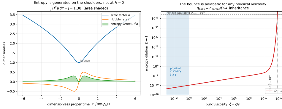
Figure 8.2: The bounce entropy budget. Left: the entropy-production kernel peaks on the shoulders of the bounce and vanishes at the turnaround; the total is tiny. Right: the dilution D - 1 versus bulk viscosity stays \lesssim 10^{-10} across the whole physical range, so \eta_{\text{child}} \approx \eta_{\text{parent}} . Reproducible as sims/src/cartasis_sims/extruder.py , figures/scripts/ch09_extruder.py (and ch09_shear.py for the shear channel).
