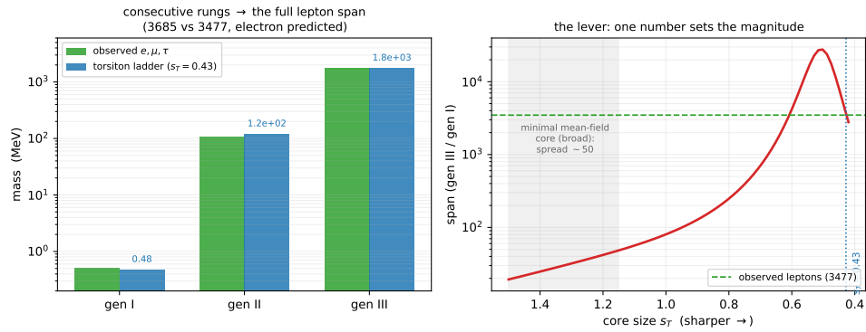
Figure 6.4: The generation hierarchy as one number—the sharpness of the mass-giving core. Left : the consecutive radial ladder n = 1, 2, 3 against a core of a single sharpness s_T reproduces the whole charged-lepton span—predicted (0.48, 121, 1777) MeV versus observed (0.51, 106, 1777), a spread of 3685 against 3477—with the electron’s tiny mass a prediction once the heaviest rung sets the scale (no exotic radial selection rule). Right : the lever. The configurational-mass span, Eq. (6.8), sweeps orders of magnitude as the core sharpens; the observed lepton spread is crossed at a plausible, sharp-but-physical core. The minimal self-consistent (mean-field) soliton digs a broad core (spread \sim 50 , shaded), so the climb to the full span is the deeper IR dynamics—one lattice-measurable quantity, the condensate profile around the torsiton (Appendix B). The hierarchy is thus not derived but reduced to a single number . Reproducible as figures/scripts/appC_generations.py .
