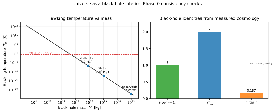
Figure 12.1: Phase-0 consistency checks, read straight off Planck cosmology. Left : the Hawking temperature T_H(M) puts the observable universe \sim 30 orders below the CMB, so the CMB is not present-horizon radiation. Right : the black-hole identities R_s/R_H = \Omega \approx 1 , maximal spin a_{\max}^* \approx 2 , and membrane filter f \approx 0.16 . Reproducible as figures/scripts/ch02_bh_first_light.py.
