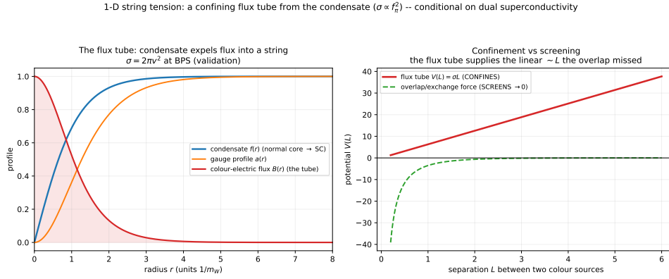
Figure 8.3: A confining flux tube from the condensate. A Nielsen–Olesen vortex squeezes colour-electric flux into a string of tension \sigma = 2\pi v^2 (the same condensate scale that sets mass), giving the linear confinement the screening overlaps cannot. Conditional on the vacuum being a dual superconductor.
