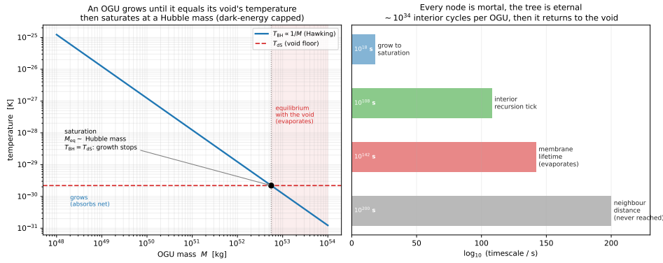
Figure 5.9: The OGU as a finite-lived recursive timeline. Left : the Hawking temperature T_{BH} \propto 1/M falls as the OGU grows toward the void’s de Sitter scale near a Hubble mass (the single-horizon heuristic; the rigorous two-horizon picture, where the cap is geometric and T_b > T_c keeps it evaporating, is Figure 5.8). Right : the timescale ladder, each step vastly longer than the last—grow ( \sim 10^{18} s) \ll interior recursion tick ( \sim 10^{108} s) \ll membrane lifetime ( \sim 10^{142} s, \sim 10^{34} interior cycles) \ll neighbour distance ( e^{1/4} horizons, never reached). Every node is mortal; the tree is eternal. Reproducible as figures/scripts/ch05_recursion.py .
