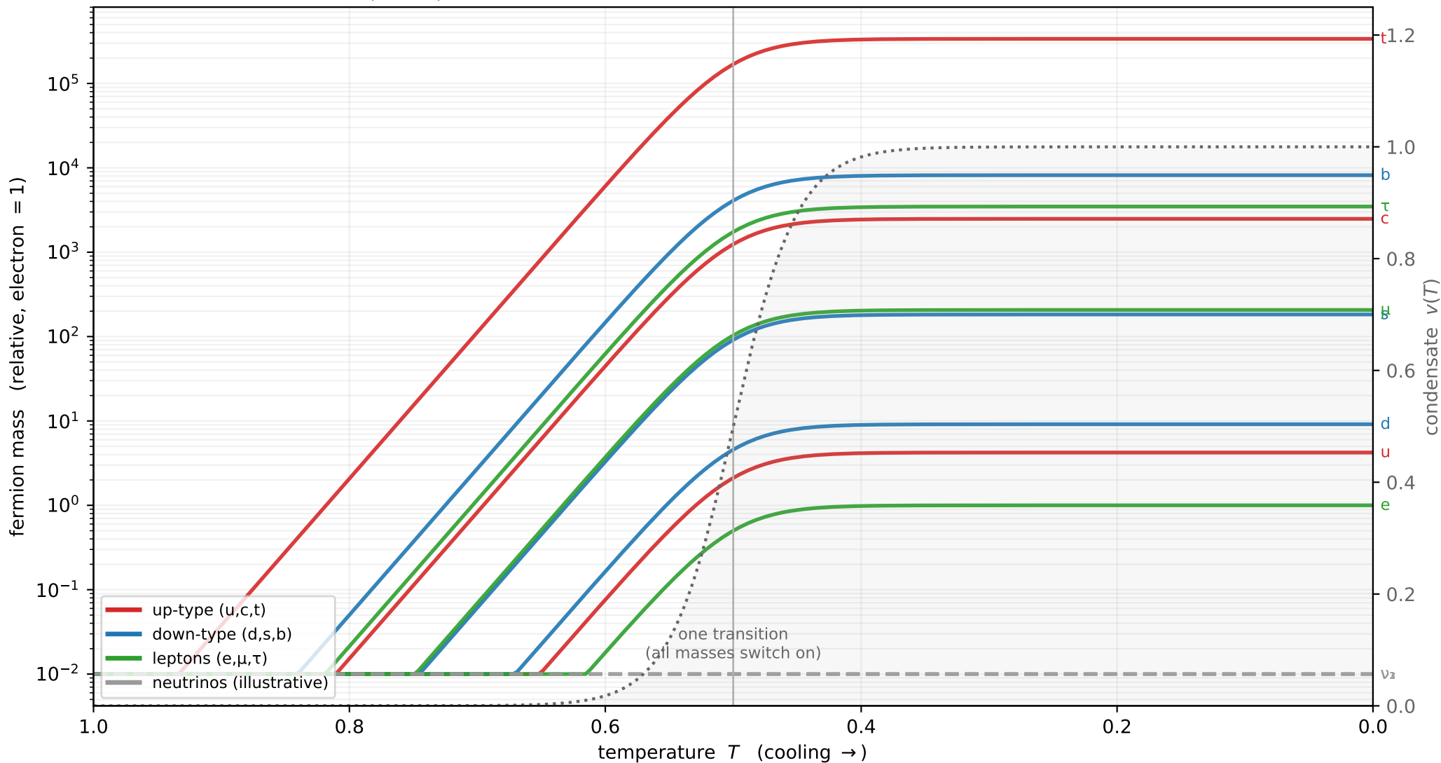
The Horizon: the twelve fermions condensing out of one chiral transition m = \Lambda c_T |O_n(s_T)|^2 — tower coupling c_T (colour) sets the bands, rung s_T sets the generations
