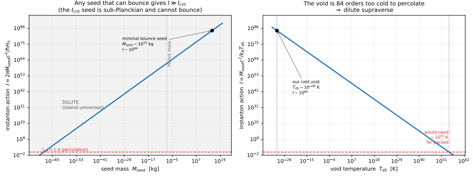
Figure 5.7: Computing the OG-nucleation instanton action, I = 2\pi M_{\text{seed}} c^2 / \hbar H_\Lambda (Equation (5.13)). Left: I versus seed mass; any seed massive enough to bounce ( M_{\text{seed}} \sim 10^{15} kg, the self-gravitating minimum) gives I \sim 10^{84} \gg I_{\text{crit}} \simeq 1.4 , the I_{\text{crit}} seed being sub-Planckian and unable to bounce. Right: I versus void temperature; the cold de Sitter void ( \sim 10^{-30} K) is eighty-four orders too cold to percolate. The verdict is robust: a dilute, eternal-inflation-like supravse of isolated island universes. Reproducible as figures/scripts/ch05_instanton.py.
