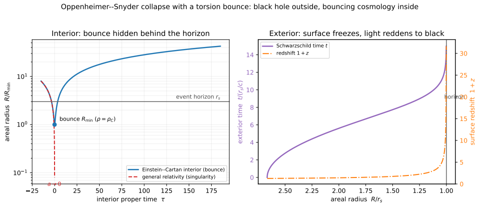
Figure 9.4: Oppenheimer–Snyder collapse with a torsion-bounce interior. Left : the surface’s areal radius collapses through the horizon and bounces at R_{\min} (blue) where general relativity reaches a singularity (red dashed). Right : from outside, the surface freezes at the horizon—Schwarzschild time t \rightarrow \infty and surface redshift 1+z \rightarrow \infty as R \rightarrow r_s . A black hole from outside; a bouncing, re-expanding cosmology from inside.
