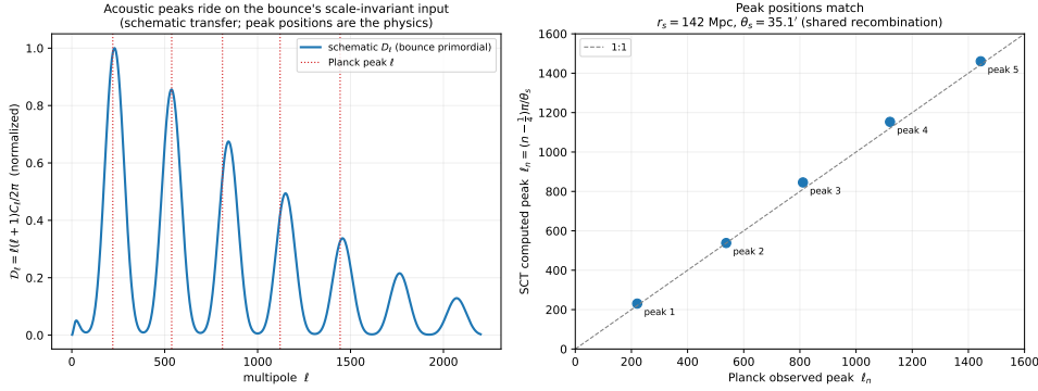
Figure 12.4: The acoustic peaks. The bounce’s scale-invariant primordial input, carried through the standard post-bounce plasma, yields a sound horizon r_s \simeq 142 Mpc and a peak series matching the observed Planck multipoles to a few percent. The peak heights are computed in Figure 12.5. Reproducible as figures/scripts/ch09_acoustic.py .
