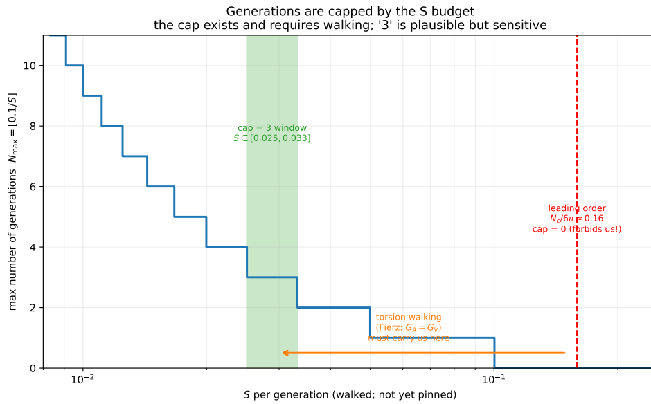
Figure 6.4: Generations as a capped ladder. The internal excitation budget is finite, so the geometric mass tower terminates—a structural reason for a small, fixed number of generations.
