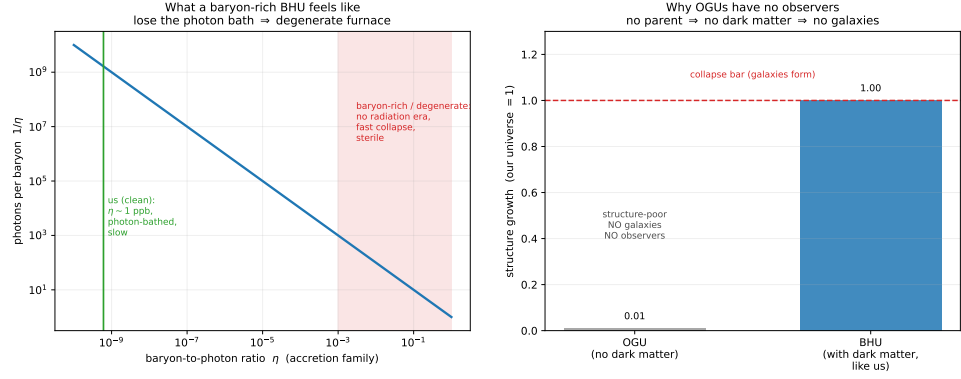
Figure 8.4: What other universe types are like. Left : along the accretion-family axis, photons per baryon 1/\eta —our clean cosmos ( \eta \sim 1 ppb) is photon-bathed and slow, while a baryon-rich one ( \eta \rightarrow 1 ) has no radiation era and collapses fast into a degenerate, sterile furnace. Right : structure growth normalised to our universe—an OGU, having no parent and so no dark matter, grows baryon-only and clears only \sim 1\% of the collapse bar, forming no galaxies. Observers live in clean-family BHU n only; the OGU root and the degenerate tail are empty by prediction.
