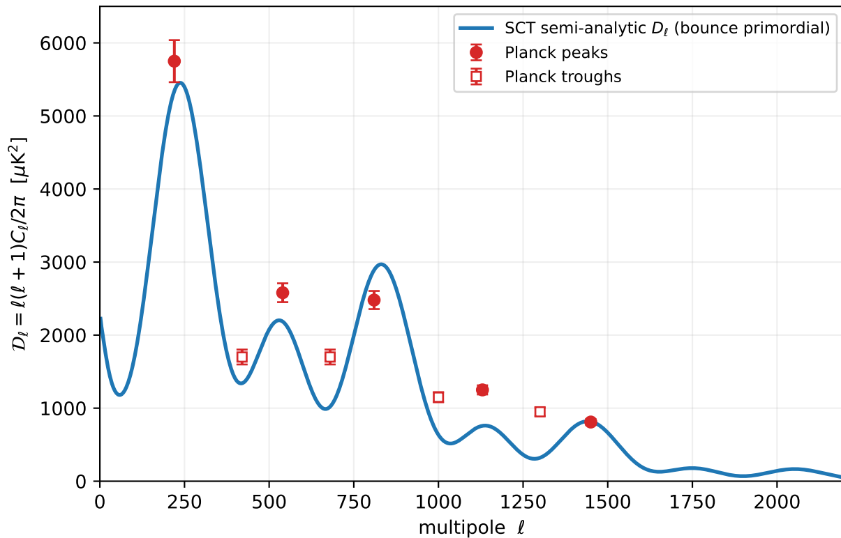
Peak heights from the bounce spectrum baryon loading + driving + Silk damping (semi-analytic)
