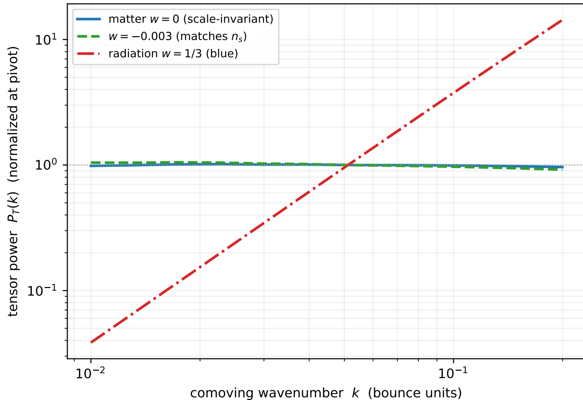
The bounce sets the primordial spectrum matter contraction \Rightarrow scale-invariant, no inflaton
