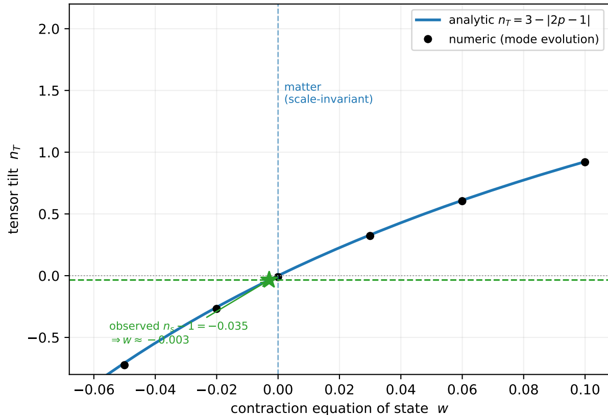
Tilt tracks the contraction scale-invariance at w = 0 ; slight red needs w \lesssim 0
