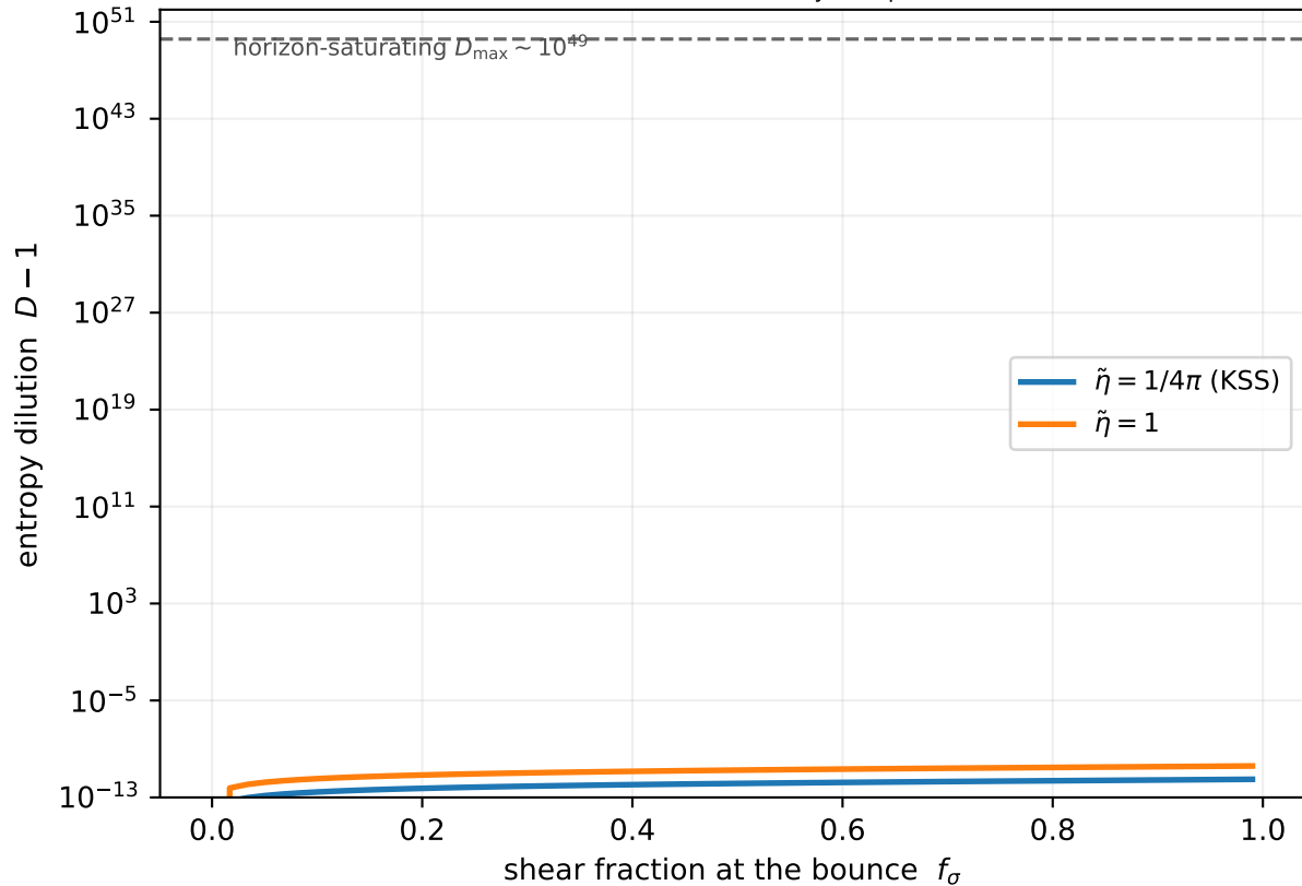
Even shear-dominated, the bounce stays adiabatic
