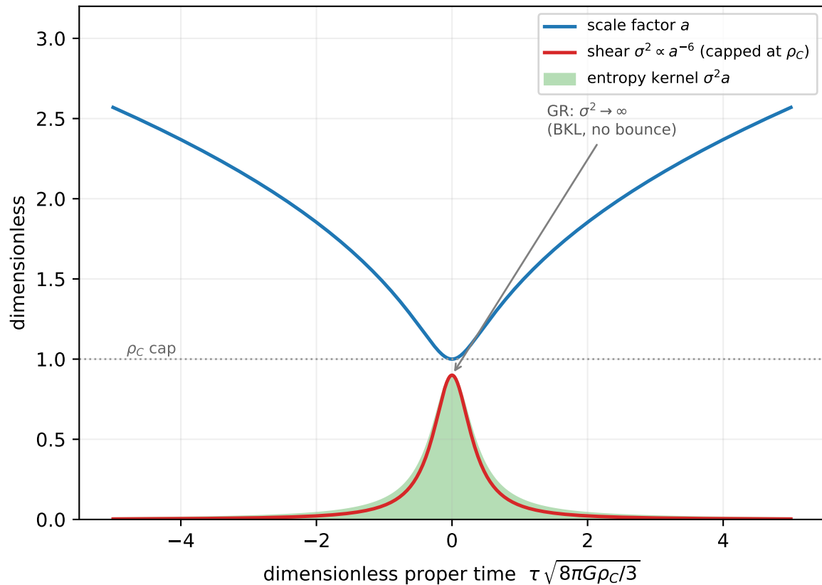
A shear-dominated bounce ( f_\sigma = 0.9 ): torsion caps the shear instead of letting it diverge
