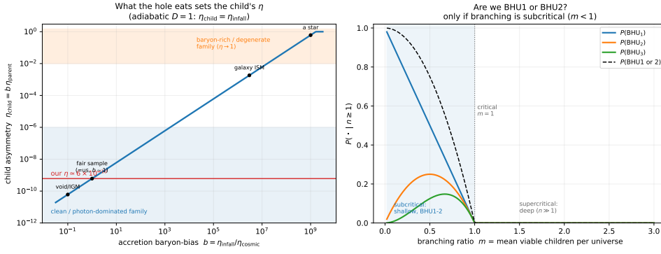
Figure 5.3: Left : the adiabatic bounce makes the child’s asymmetry equal to that of the accreted material, \eta_{\text{child}} = b \eta_{\text{parent}} (Equation (5.4)), splitting each lineage into a clean, photon-dominated family and a baryon-rich, degenerate one. Our \eta \simeq 6 \times 10^{-10} places our progenitor at a fair-sample accretor ( b \sim 1 ), not a star-fed one. Right : given n \geq 1 , P(\text{BHU}_n) \propto m^n ; we are likely \text{BHU}_{1-2} only if the branching ratio is subcritical ( m < 1 ), otherwise the population is deep. Reproducible as figures/scripts/ch05_accretion.py.
