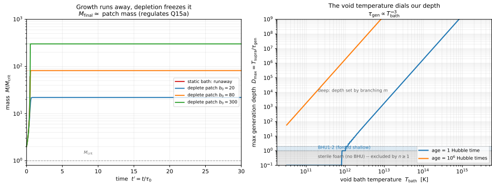
Figure 5.4: Left: growth trajectories from (5.5). In a static bath the hole runs away (finite-time blow-up); depleting a finite local patch freezes it at M_{final} \sim the patch mass—the regulator that keeps universe-holes finite. Right: the maximum generation depth D_{max} = T_{supra}/\tau_{gen} versus the void bath temperature ( \tau_{gen} \propto T_{bath}^{-3} ), for two supravse ages. Below the sterile line no BHU forms (excluded by our existence); a narrow band gives the forced-shallow BHU 1-2 ; above it the depth is large and set by the branching ratio.
