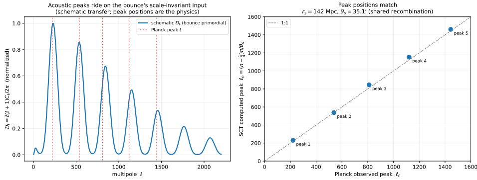
Figure 9.9: Left : a schematic CMB temperature spectrum—the bounce’s scale-invariant primordial input times a damped acoustic transfer—with the observed Planck peak multipoles marked (dotted); the peaks ride at the right places. Right : the SCT-computed peak positions \ell_n = (n - \frac{1}{4})\pi/\theta_s , from the sound horizon r_s \simeq 142 Mpc, against the Planck peaks—on the 1:1 line, because the pre-recombination acoustics are shared with \Lambda CDM. The schematic spectrum is illustrative; the peak positions are the physics. Reproducible as figures/scripts/ch09_acoustic.py .
