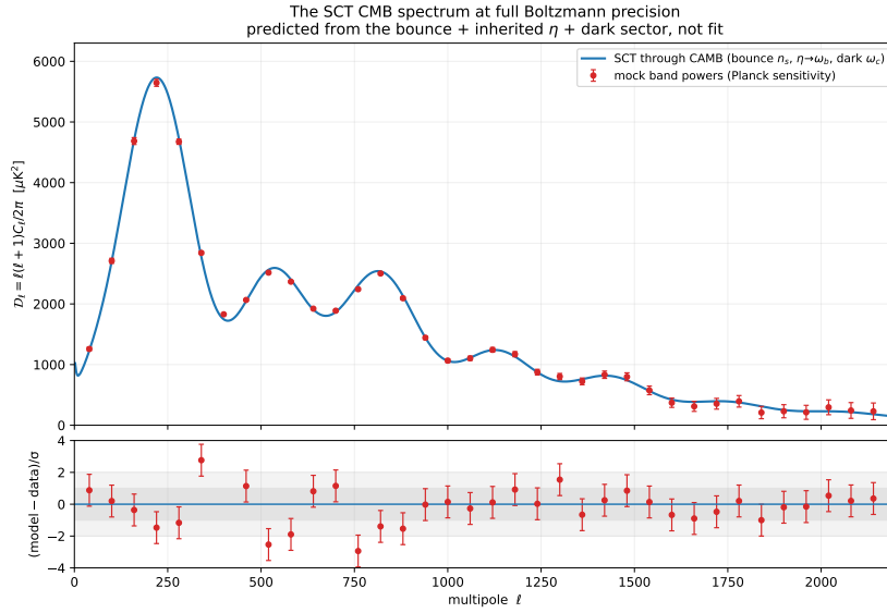
Figure 9.11: The SCT CMB spectrum at full Boltzmann precision. Top : the TT spectrum from CAMB for the SCT parameter set (bounce n_s , \eta \rightarrow \omega_b , dark-sector \omega_c ), against mock band powers at Planck sensitivity (the model binned with realistic cosmic-variance+noise errors and scatter—a fair “what Planck would measure,” not hand-entered data). Bottom : residuals in units of the band-power error, consistent with \sim 1\sigma scatter. Because the SCT inputs coincide with the Planck best fit, the match is by construction; the independent result is that the inherited \eta predicts the \omega_b that sets the peak heights.
