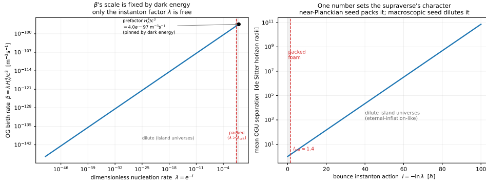
Figure 5.6: Pinning the OG birth rate. Left : \beta = \lambda H_\Lambda^4 / c^3 ; the prefactor ( \sim 4 \times 10^{-97} \text{ m}^{-3} \text{ s}^{-1} ) is fixed by the observed dark energy, leaving only the instanton factor \lambda = e^{-I} free. Right : the mean OGU separation versus the instanton action I ; the de Sitter percolation threshold I_{\text{crit}} \simeq 1.4 splits a packed polygonal foam (near-Planckian seed) from a dilute scatter of island universes (macroscopic seed). Reproducible as figures/scripts/ch05_birthrate.py.
