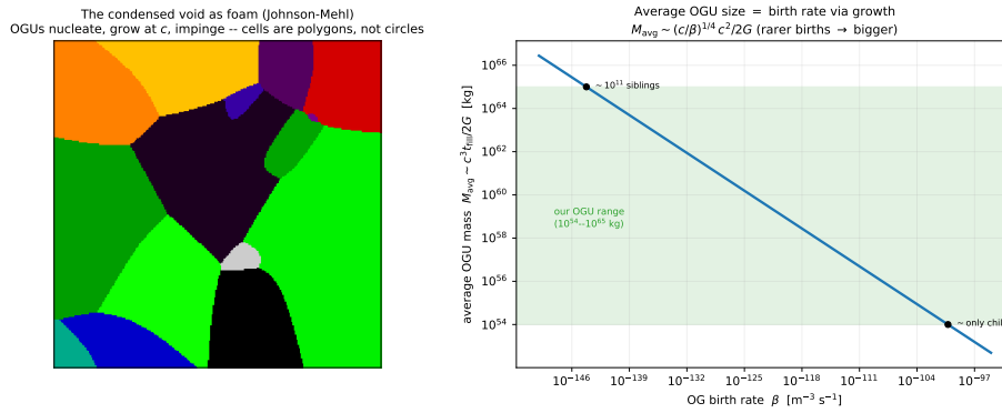
Figure 5.11: Left : the condensed void as a Johnson–Mehl foam—OGUs nucleate, grow at the causal speed c , and impinge, tiling the void into curved polygons (an isolated young OGU would be round). Right : the average OGU mass set by the birth rate, (5.17): rarer births give fewer, larger universes. Our OGU’s plausible mass range ( 10^{54} – 10^{65} kg, Section 5.7.5) maps to a band of birth rates. Reproducible as figures/scripts/ch05_voidfoam.py .
