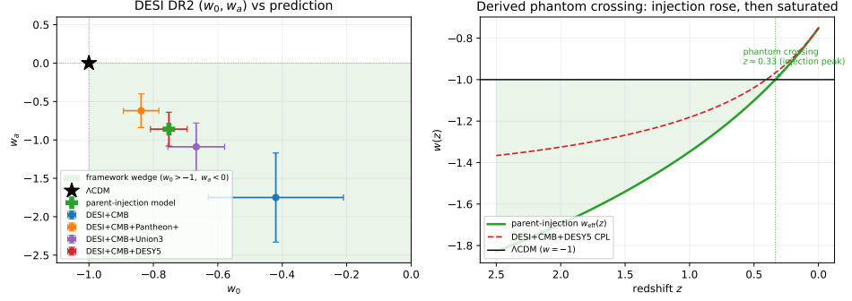
Figure 6.2: Dark energy as parent accretion vs DESI DR2. Left : the four DESI DR2 ( w_0, w_a ) fits all fall in the framework’s wedge ( w_0 > -1, w_a < 0 , shaded); \Lambda CDM (star) sits at its corner, disfavoured at 2.8\text{--}4.2\sigma . Right : the peaked-injection w_{eff}(z) of (6.1) crosses w = -1 at the injection peak z_{cross} \approx 0.33 (shaded: phantom epoch), tracking the DESI CPL reconstruction through the constrained range. Values flagged for verification against the published tables.
