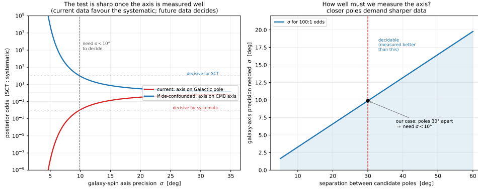
Figure 8.2: The decisive shared-axis test as a two-hypothesis comparison. Left: posterior odds (SCT:systematic) versus the precision \sigma to which the galaxy-spin axis is measured. With today’s geometry (axis on the Galactic pole) the odds favour the systematic (red); a de-confounded measurement with the axis on the CMB axis would favour SCT (blue); either way \sigma \lesssim 10^\circ is needed to decide. Right: because the candidate poles are only \sim 30^\circ apart, the required precision is \sim 10^\circ —closer poles would demand sharper data. The discriminant is whether a well-measured spin axis favours the CMB axis or the Galactic pole.
