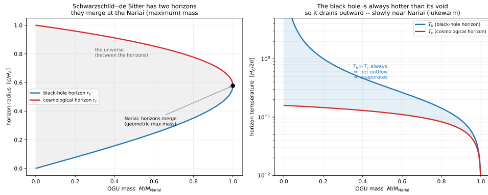
Figure 5.8: Why an OGU evaporates though it looks “in equilibrium.” Left: Schwarzschild–de Sitter has two horizons—the black-hole horizon r_b and the cosmological horizon r_c , the universe living between them—which merge at the Nariai (maximum) mass: the growth cap is geometric . Right: their temperatures, T_b > T_c for every sub-Nariai mass (equal only at the unstable Nariai point), so the black hole is always hotter than its own void and drains outward—slowly near Nariai (a lukewarm plateau that mimics equilibrium but is not it). Reproducible as figures/scripts/ch05_sds.py .
