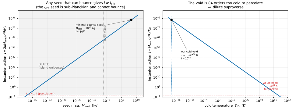
Figure 5.7: Computing the OG-nucleation instanton action, I = 2\pi M_{\text{seed}} c^2 / \hbar H_\Lambda (Equation (5.11)). Left: I versus seed mass; any seed massive enough to bounce ( M_{\text{seed}} \sim 10^{15} kg, the self-gravitating minimum) gives I \sim 10^{84} \gg I_{\text{crit}} \simeq 1.4 , the I_{\text{crit}} seed being sub-Planckian and unable to bounce. Right: I versus void temperature; the cold de Sitter void ( \sim 10^{-30} K) is eighty-four orders too cold to percolate. The verdict is robust: a dilute, eternal-inflation-like supaverse of isolated island universes. Reproducible as figures/scripts/ch05_instanton.py.
