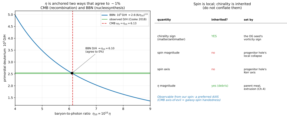
Figure 8.3: Left : \eta is anchored two independent ways that agree to \sim 1\% —the CMB-fixed \omega_b and BBN deuterium—so the baryon asymmetry is secure despite the parent-Hawking CMB reading (which leaves BBN untouched). Right : spin versus chirality. The chirality sign is inherited (pure lineages); spin magnitude and axis are local (the progenitor hole’s Kerr spin), so \text{spin}_{\text{us}} \neq \text{spin}_{\text{OGU}} . The observable from our spin is a preferred axis, shared by the CMB anomalies and the galaxy-spin asymmetry.
