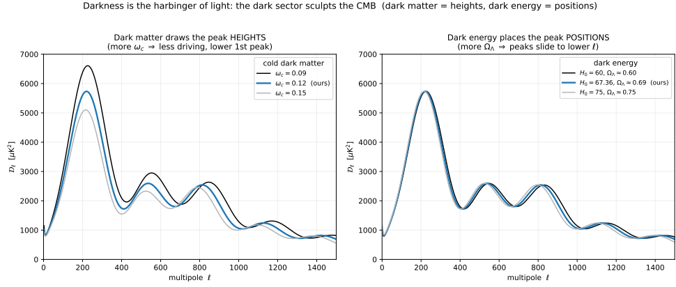
Figure 9.12: The dark sector sculpts the CMB along two axes. Left : varying the cold-dark-matter density \omega_c (ours in blue) changes the peak heights —more dark matter damps the driving and lowers the first peak. Right : varying the dark energy \Omega_\Lambda (through H_0 at fixed physical densities) slides the peak positions . In SCT both are the parent’s gravity felt before its light (Section 6.2.4), so the darkness in our metric now is what shaped the oldest light: darkness is the harbinger of light.
