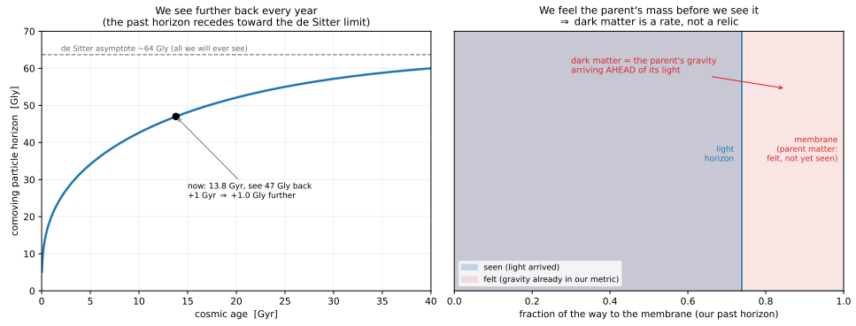
Figure 6.1: The dark sector as look-back into the parent. Left : the comoving particle horizon grows with cosmic age toward a de Sitter asymptote ( \simeq 64 Gly); we see \sim 1 Gly further back per additional Gyr, so parent-injected matter becomes visible only as the past horizon recedes out to it. Right : the parent’s mass is already in our metric (felt as dark matter, red) while its light is still climbing in from the past horizon (seen, blue)—gravity leads light. Dark matter is the parent’s pull arriving ahead of its image.
