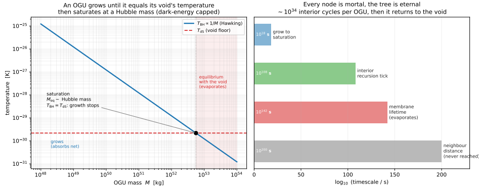
Figure 5.9: The OGU as a finite-lived recursive timeline. Left : the Hawking temperature T_{\text{BH}} \propto 1/M falls as the OGU grows toward the void’s de Sitter scale near a Hubble mass (the single-horizon heuristic; the rigorous two-horizon picture, where the cap is geometric and T_b > T_c keeps it evaporating, is Figure 5.8). Right : the timescale ladder, each step vastly longer than the last—grow ( \sim 10^{18} s) \ll interior recursion tick ( \sim 10^{108} s) \ll membrane lifetime ( \sim 10^{142} s, \sim 10^{34} interior cycles) \ll neighbour distance ( e^{1/4} horizons, never reached). Every node is mortal; the tree is eternal. Reproducible as figures/scripts/ch05_recursion.py .
