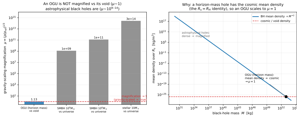
Figure 13.1: Gravity-scaling magnification \mu = (\rho/\rho_{\text{ref}})^{1/3} . Left : an OGU (horizon mass, mean density = cosmic) sits at \mu \simeq 1 —gravity-scaled coordinates equal true coordinates at the OGU/void level— while astrophysical black holes, far denser than their host, magnify by 10^9 – 10^{14} . Right : the black-hole mean density crosses the cosmic/void line precisely at the horizon mass, which is why an OGU scales to unity (the R_s = R_H identity). Reproducible as figures/scripts/ch10_gravity_scale.py.
