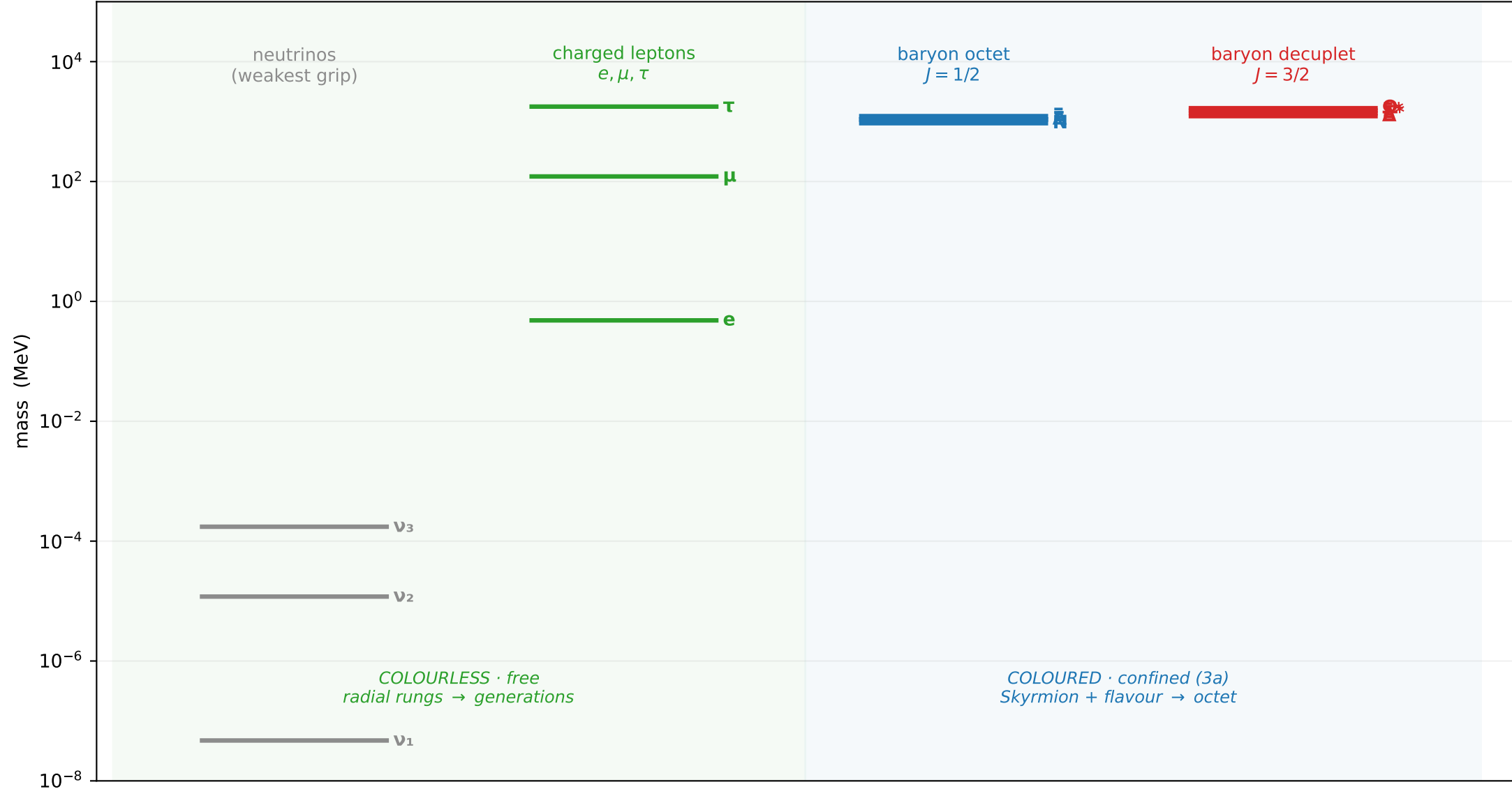
The observable fermion spectrum from ONE chiral soliton leptons = colourless rungs (3c) · baryons = coloured Skyrmions (3b) · quarks confined within (3a)
