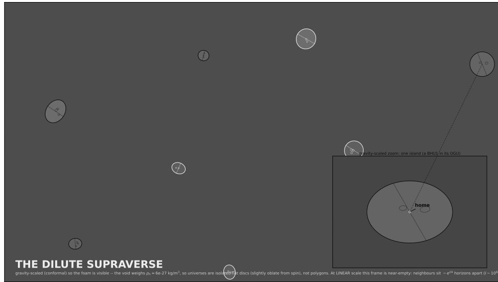
Figure 10.4: The dilute supraverse, gravity-scaled (sizes and spacings illustrative, not linear). The weighted void ( \rho_\Lambda \sim 6 \times 10^{-27} \text{ kg m}^{-3} , faintly speckled with zero-point energy) dominates; universes are sparse, round , isolated islands (gravity wells with chirality-toned Cartasis membranes, faint nested BHU children). The inset zooms one, marking home . At a literal linear scale the frame would be near-empty—neighbours lie \sim e^{1/4} horizons apart—so the void’s weight keeps the islands round while the dilution makes the true gaps astronomically larger than drawn.
