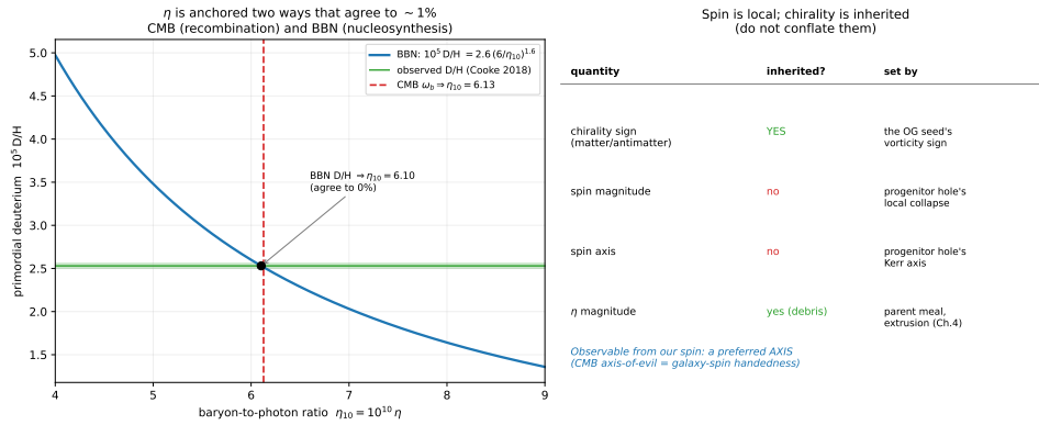
Figure 8.2: Left: \eta is anchored two independent ways that agree to \sim 1\% —the CMB-fixed \omega_b and BBN deuterium—so the baryon asymmetry is secure despite the parent-Hawking CMB reading (which leaves BBN untouched). Right: spin versus chirality. The chirality sign is inherited (pure lineages); spin magnitude and axis are local (the progenitor hole’s Kerr spin), so \text{spin}_{\text{us}} \neq \text{spin}_{\text{OGU}} . The observable from our spin is a preferred axis, shared by the CMB anomalies and the galaxy-spin asymmetry.
