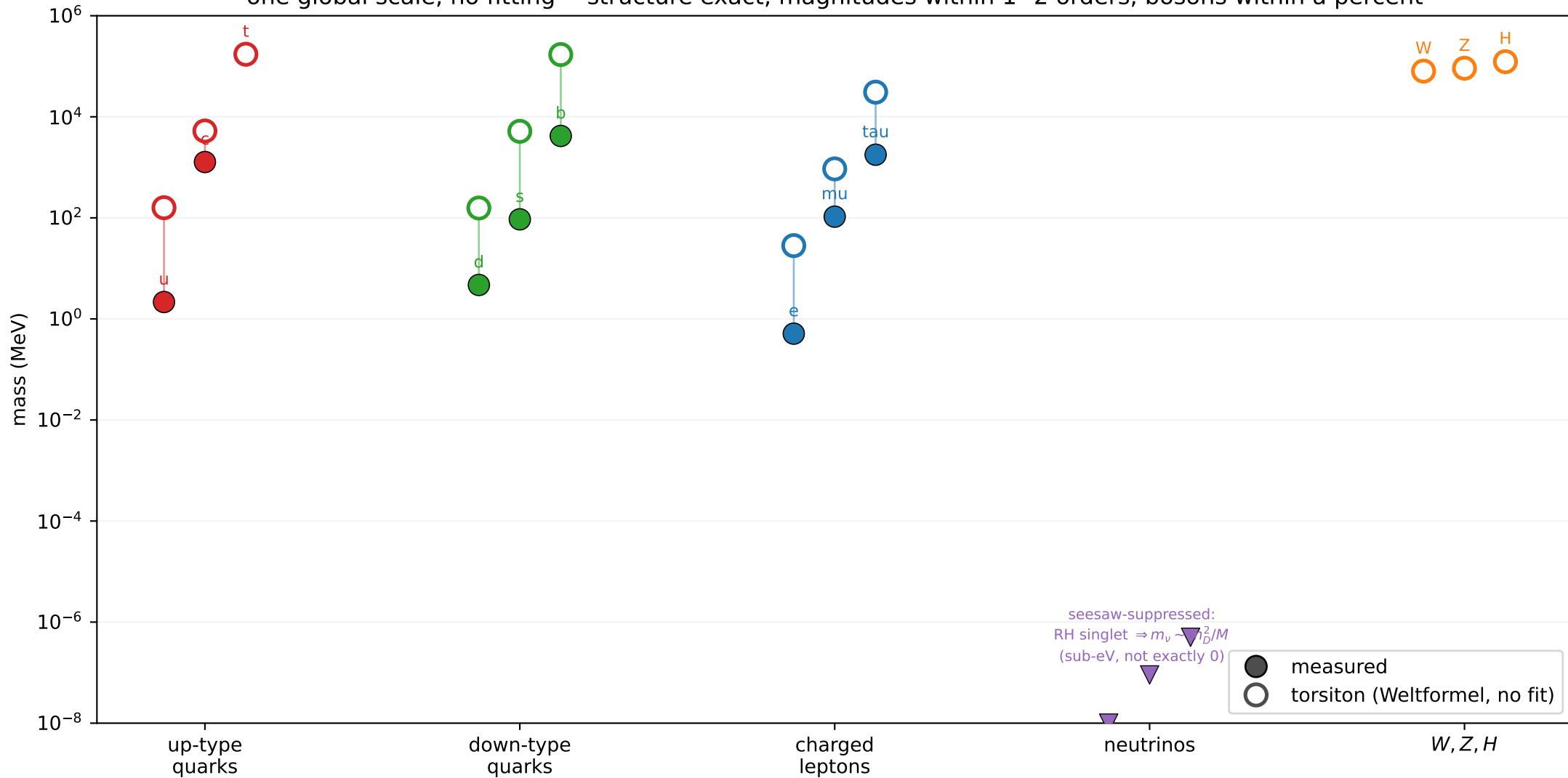
The Weltformel spectrum: all 15 elementary masses from the equations one global scale, no fitting -- structure exact, magnitudes within 1--2 orders, bosons within a percent
