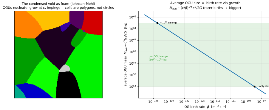
Figure 5.7: Left : the condensed void as a Johnson-Mehl foam—OGUs nucleate, grow at the causal speed c , and impinge, tiling the void into curved polygons (an isolated young OGU would be round). Right : the average OGU mass set by the birth rate, (5.12): rarer births give fewer, larger universes. Our OGU’s plausible mass range ( 10^{54} – 10^{65} kg, Section 5.7.5) maps to a band of birth rates. Reproducible as figures/scripts/ch05_voidfoam.py.
