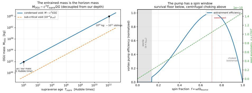
Figure 5.6: Left : the entrained OGU mass is the horizon mass of its causal patch, M_{\text{OGU}} \sim c^3 T_{\text{supra}} / 2G (Equation (5.11)): our mass at one Hubble time, \sim 10^{65} kg (and \sim 10^{11} siblings) at \sim 10^{12} Hubble times; a sub-critical void gives less. Right : the vortex pump has a spin window—a survival floor f_{\text{min}} below (sterile) and centrifugal choking near extremal above—so genesis favours an intermediate spin sweet spot. The headline mass relation is robust; the efficiency shape is illustrative. Reproducible as figures/scripts/ch05_genesis.py.
