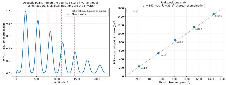
Figure 9.9: Left: a schematic CMB temperature spectrum—the bounce’s scale-invariant primordial input times a damped acoustic transfer—with the observed Planck peak multipoles marked (dotted); the peaks ride at the right places. Right: the SCT-computed peak positions \ell_n = (n - \frac{1}{4})\pi/\theta_s , from the sound horizon r_s \simeq 142 Mpc, against the Planck peaks—on the 1:1 line, because the pre-recombination acoustics are shared with \Lambda CDM. The schematic spectrum is illustrative; the peak positions are the physics. Reproducible as figures/scripts/ch09_acoustic.py .
