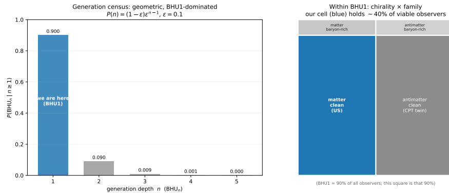
Figure 10.4: The supraverse census of viable observers. Left : the generation tower is geometric and first-generation-dominated; we are in the n = 1 bar. Right : within that generation, our cell (matter, clean family) holds \sim 40\% of viable observers, with an identical antimatter CPT twin. Our footprint is the typical, dominant cell. Reproducible as figures/scripts/ch08_census.py .
