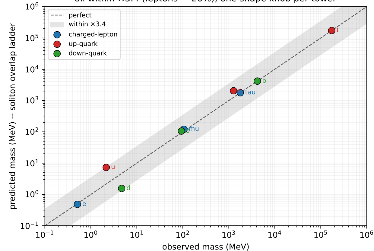
9 charged fermions from the overlap ladder all within \times 3.4 (leptons \sim 20\% ), one shape knob per tower
