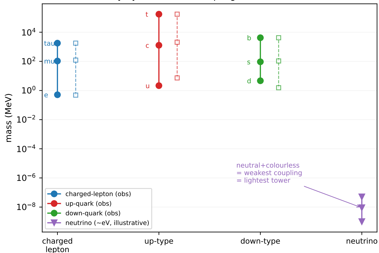
The four towers: solid=observed, dashed=ladder hierarchy by condensate coupling; neutrinos at the floor
