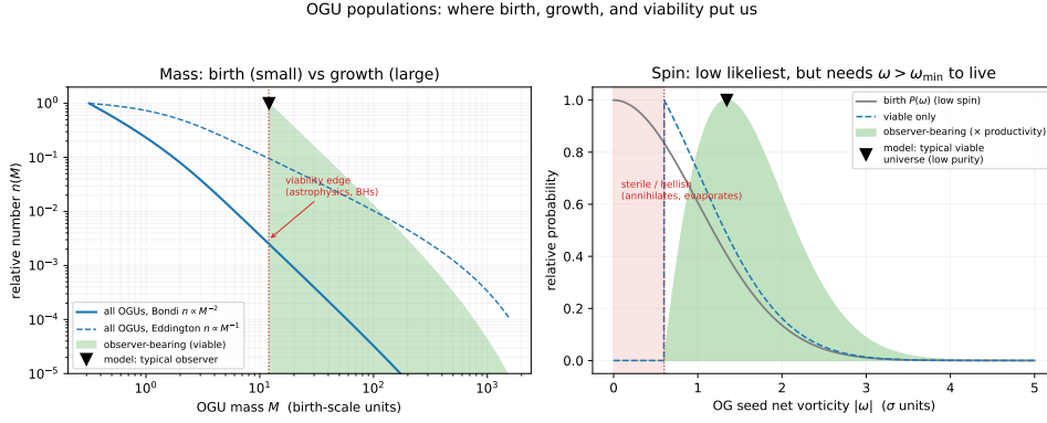
Figure 5.1: OGU populations from first competition. Left : the mass distribution (5.1)—births (small) versus runaway growth (large) give a power law n(M) \propto M^{-\delta} ; a viability cut selects observer-bearing universes, which peak just above the edge—where the framework predicts a typical observer sits. Right : the spin distribution (Section 5.7.3)—low net vorticity is likeliest, but below \omega_{\min} baryogenesis fails and the universe is sterile, so viable universes sit just above threshold (low purity, small \eta ). The markers are the model’s predicted typical location, not independent measurements of our universe; the horizontal axes are in model units ( M_0 and \sigma ). Generated by figures/scripts/ch05_distributions.py .
