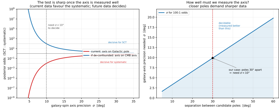
Figure 8.2: The shared-axis test as a two-hypothesis comparison—a precision question, since the candidate poles are close. Left : posterior odds (CMB axis : Galactic pole) versus the precision \sigma to which the galaxy-spin axis is measured. With today’s geometry (axis on the Galactic pole) the odds favour the systematic (red); a de-confounded measurement with the axis on the CMB axis would favour SCT (blue); either way \sigma \lesssim 10^\circ is needed to resolve the two. Right : because the candidate poles are only \sim 30^\circ apart, the required precision is \sim 10^\circ —closer poles would demand sharper data. A null or a Galactic-pole result is inconclusive (a low-spin parent is the typical case); the strong outcomes are a galaxy axis that agrees with the CMB axis (confirmation) or two clean axes that disagree (falsification).
