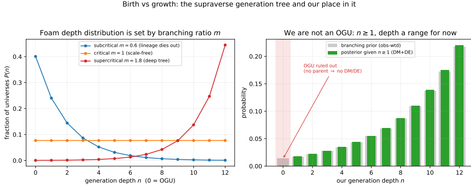
Figure 5.2: Where our universe sits in the generation tree. Left : the depth distribution (5.2) for sub-, near-, and super-critical branching m (the super-critical pile-up at the right edge reflects the hard truncation D used for illustration; a soft viability cutoff rounds it). Right : our posterior. The observation that we have dark matter and dark energy—both requiring a parent—zeroes the n = 0 (OGU) bin: we are not an original-generation universe. Generated by figures/scripts/ch05_population.py.
