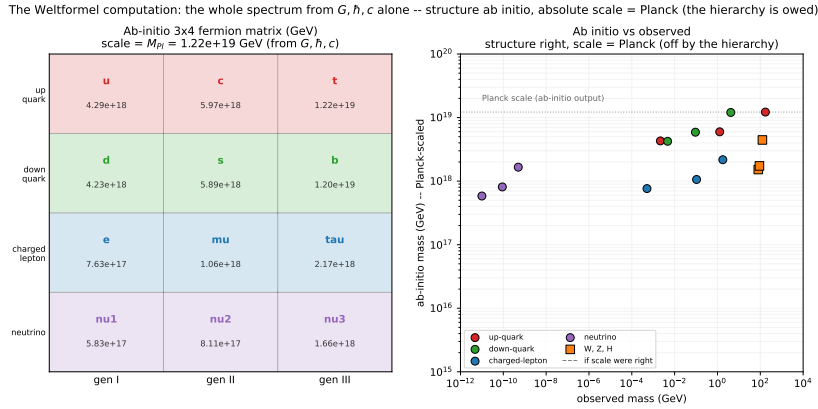
Figure 9.2: The Weltformel matrix. The full 3 \times 4 fermion spectrum (and W, Z, H ) computed from G, \hbar, c and the charge/colour handles alone—no Yukawa, no \nu , no fitted well. The structure is right (three generations, four towers; quarks above leptons; the neutrino the lightest, forced to zero in the singlet limit; gen III heaviest). The absolute scale is the Planck mass: every entry is \sim 10^{17} too heavy.
