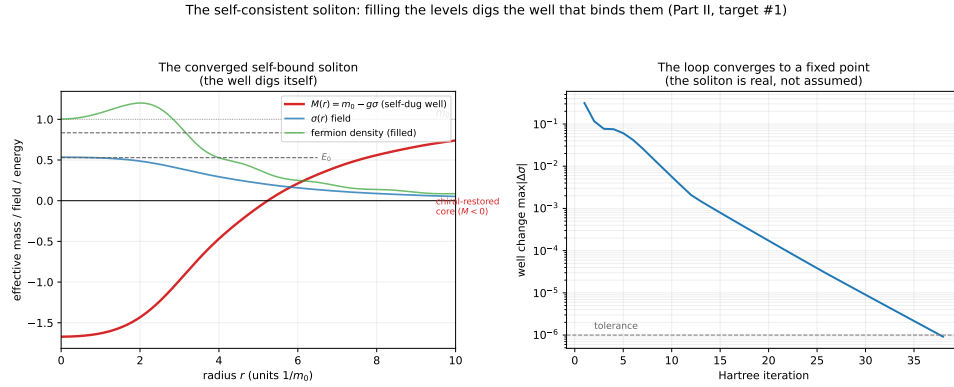
Figure 6.1: The self-consistent gravity–torsion soliton. The Hartree loop (levels \rightarrow density \rightarrow four-fermion field \rightarrow well) converges to a genuine self-bound profile: the torsiton exists as a solution, not a postulate. Reproducible from sims/src/cartasis_sims/self_consistent.py .
