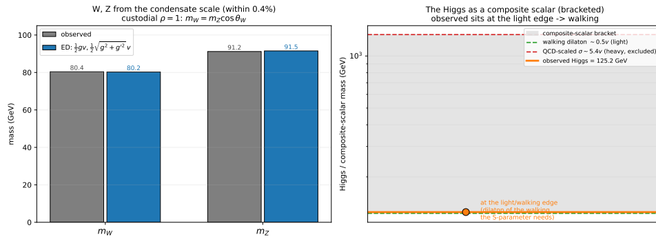
Figure 8.6: W, Z , and Higgs in the composite/walking reading. m_W, m_Z follow from the condensate scale and the gauge couplings (within 0.4%), with custodial \rho = 1 a genuine prediction. The Higgs is a composite scalar; the observed 125 GeV sits at the light, walking-dilaton edge, far from the excluded heavy-sigma.
