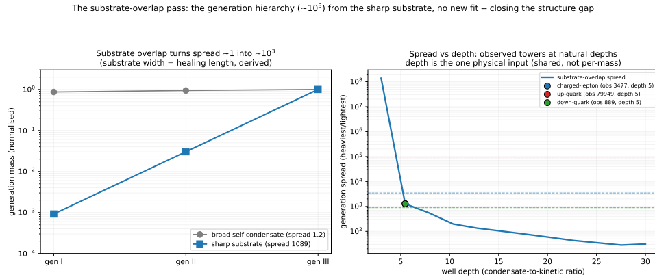
Figure 6.4: The substrate-overlap pass. Overlapping each generation with the sharply localized substrate (width = the well's healing length, derived) rather than the soliton's broad self-condensate turns the spread from \sim 1 into \sim 10^3 : the arithmetic level ladder becomes the observed geometric mass hierarchy, with no new fit.
