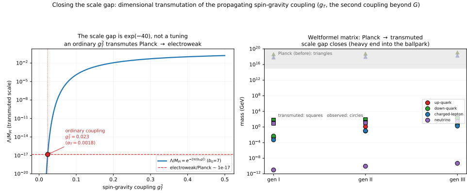
Figure 9.3: Closing the scale gap by dimensional transmutation. The Planck-to-electroweak ratio is e^{-40} , the exponential of an ordinary coupling: a propagating spin-gravity coupling g_T^2 \sim 0.02 , asymptotically free, condenses at the electroweak scale. Rescaling the Weltformel matrix from M_{Pl} to \Lambda brings the heavy end into the observed ballpark.
