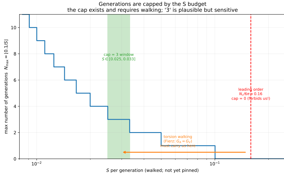
Figure 6.3: Generations as a capped ladder. The internal excitation budget is finite, so the geometric mass tower terminates—a structural reason for a small, fixed number of generations rather than an arbitrary one.
