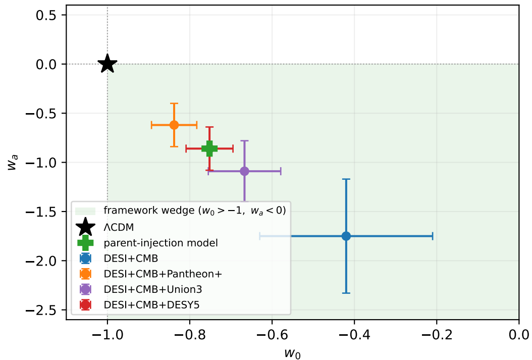
DESI DR2 ( w_0, w_a ) vs prediction
