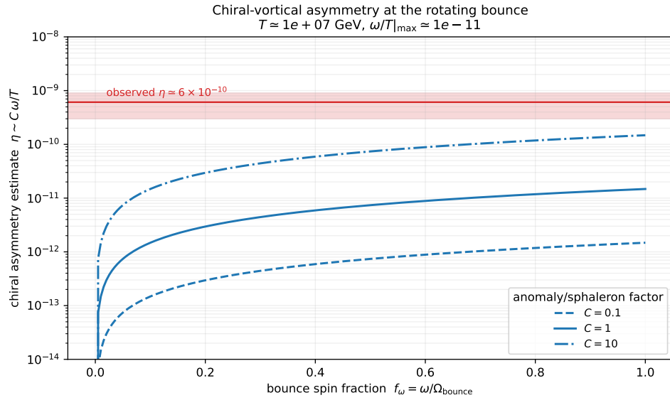
Figure 4.1: The chiral-vortical viability check at the rotating bounce. The bare small parameter \omega/T \sim 10^{-11} (maximal spin, \rho_C = 10^{50} \text{ kg m}^{-3} ) sits within \sim 1.6 orders of the observed \eta_{\text{obs}} \simeq 6.1 \times 10^{-10} : the mechanism is in the right ballpark but generically undershoots, requiring C \cdot f_\omega \simeq 41 (Eq. 4.3). The maximal-spin value is a ceiling —no seed vorticity can exceed it—so the factor must come from the anomaly/sphaleron coefficient C , not from a faster spin. Generated by figures/scripts/ch04_cve_filter.py .
