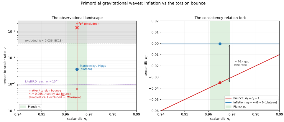
Figure 7.1: Primordial gravitational waves as the inflation-versus-bounce fork. Left : the (n_s, r) landscape—the Planck n_s band, the current bound r < 0.036 , LiteBIRD’s forecast reach \sigma_r \sim 10^{-3} , and the inflation menu (plateau models within reach; m^2\phi^2 excluded). The bounce sits at n_s \simeq 0.965 with r not fixed by a consistency relation—the simplest version is excluded at r \gtrsim 1 and a cured one drops low. Right : the tilt fork that does not need r ’s uncertain magnitude— inflation puts n_T = -r/8 \approx 0 , the bounce puts n_T = n_s - 1 \simeq -0.035 , a \sim 70\times gap at the observed n_s . Reproducible as figures/scripts/ch07_tensor_r.py.
