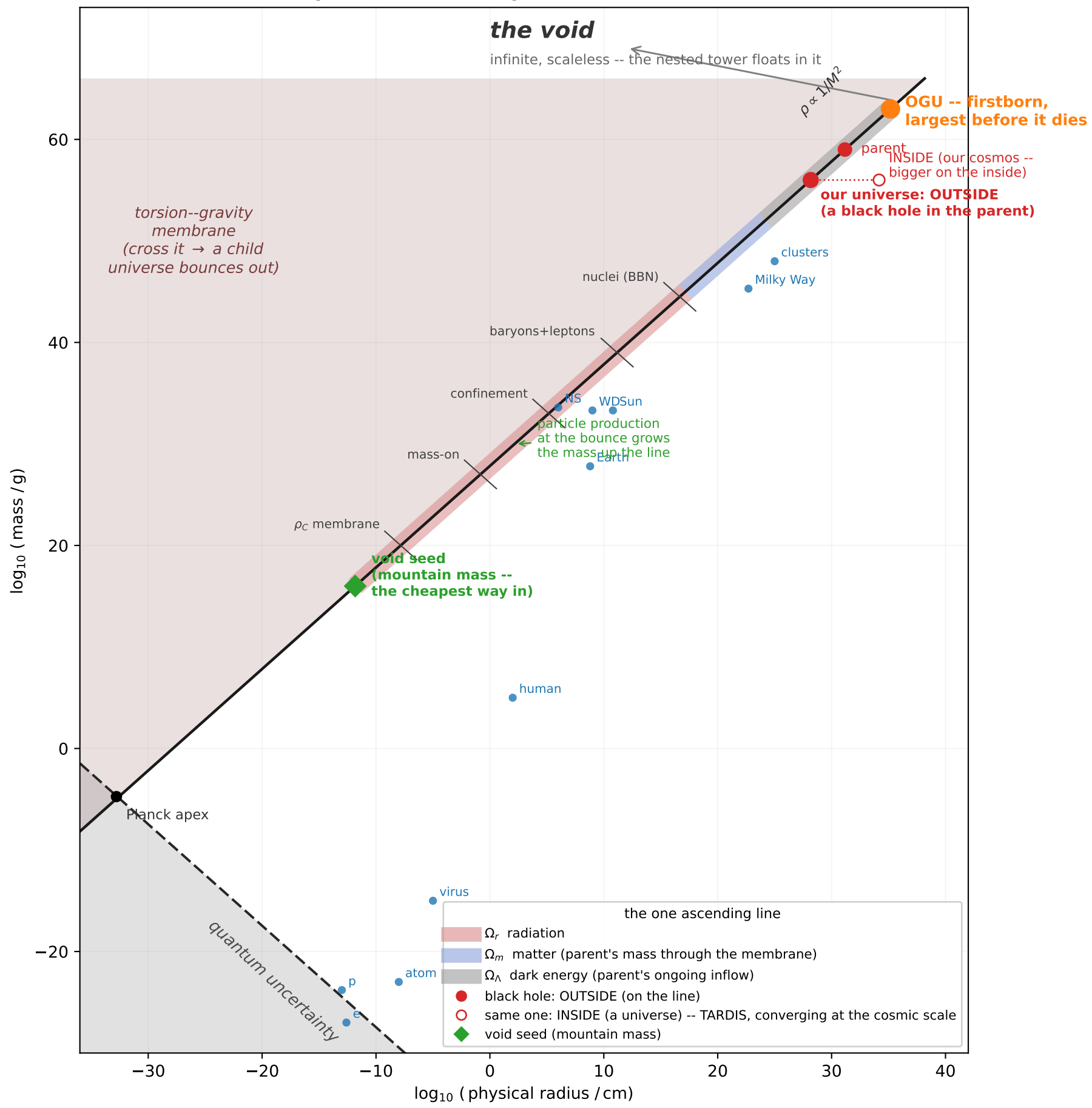
The Eternal Dawn mass--radius diagram one ascending line: void seed → genesis → us → OGU, then the void
