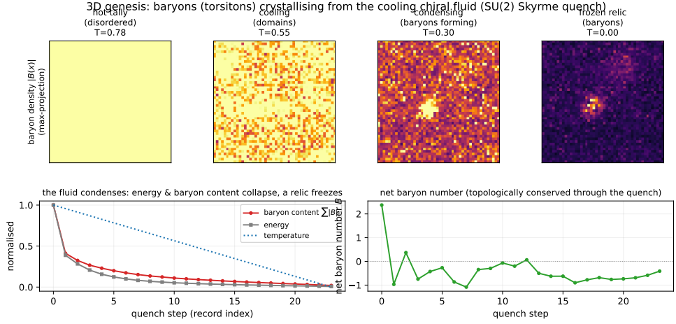
Figure 7.2: Stage 2, in three dimensions: torsitons crystallising from the cooling chiral field. The structureless hot plasma (left) freezes into localized, self-bound knots (right) as the temperature drops through the condensation threshold—matter condensing out of the field, not created from nothing. The defect count follows Kibble–Zurek. Reproducible as figures/scripts/genesis_quench3d.py .
