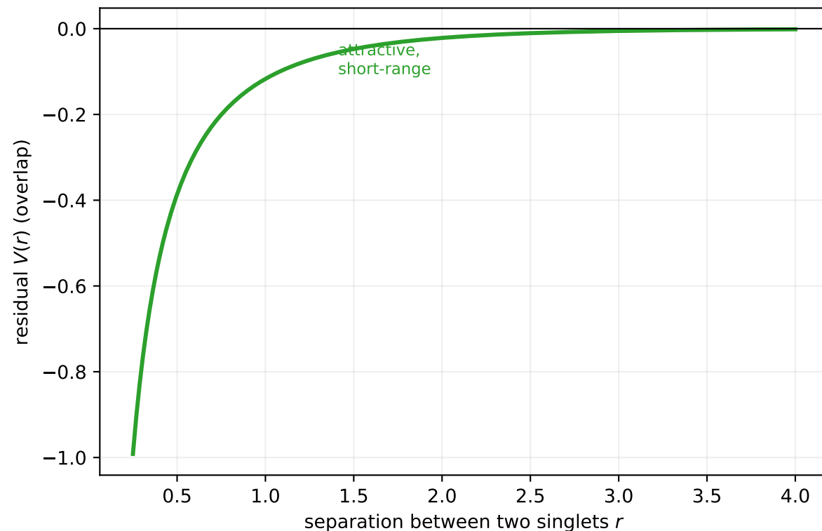
Residual force from the overlap of two singlets (the nuclear-force analogue, \sigma -exchange)
