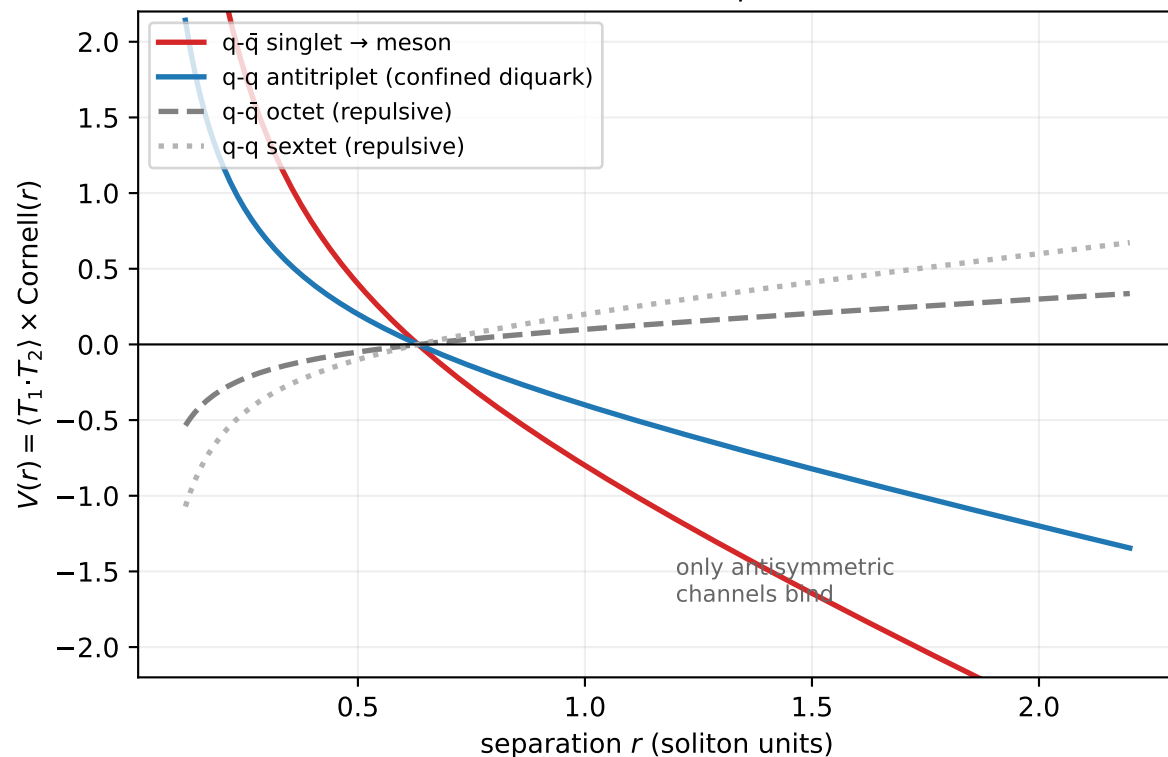
Colour-channel forces (factors RIGOROUS; shape modelled)
