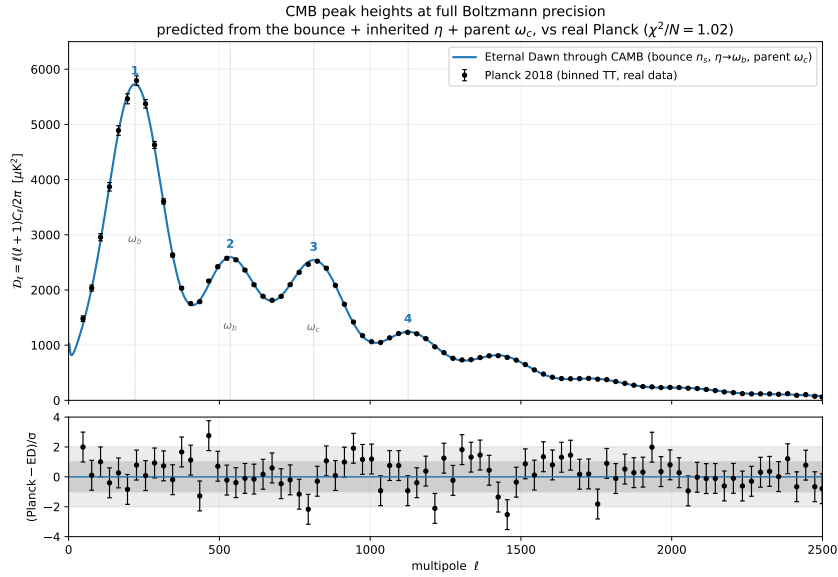
Figure 8.5: The peak heights , at full Boltzmann precision, against the real Planck 2018 binned TT spectrum. The standard recombination transfer (CAMB), fed an Eternal Dawn parameter set whose values are sourced — n_s from the bounce, \omega_b from the inherited \eta , \omega_c from the parent’s projected mass—reproduces the measured spectrum at \chi^2/N \simeq 1.0 over 83 band powers (residuals, lower panel, scatter within \pm 2\sigma ). The first peak’s height fixes the baryon density (the odd/even ratio D_1/D_2 \simeq 2.2 ), the third peak the dark-matter density ( D_1/D_3 \simeq 2.3 ); \omega_c/\omega_b \simeq 5.4 is the baryon fraction f \approx 1/6 that the membrane filter (§8.5) must derive. Reproducible as figures/scripts/ch09_peak_heights.py.
