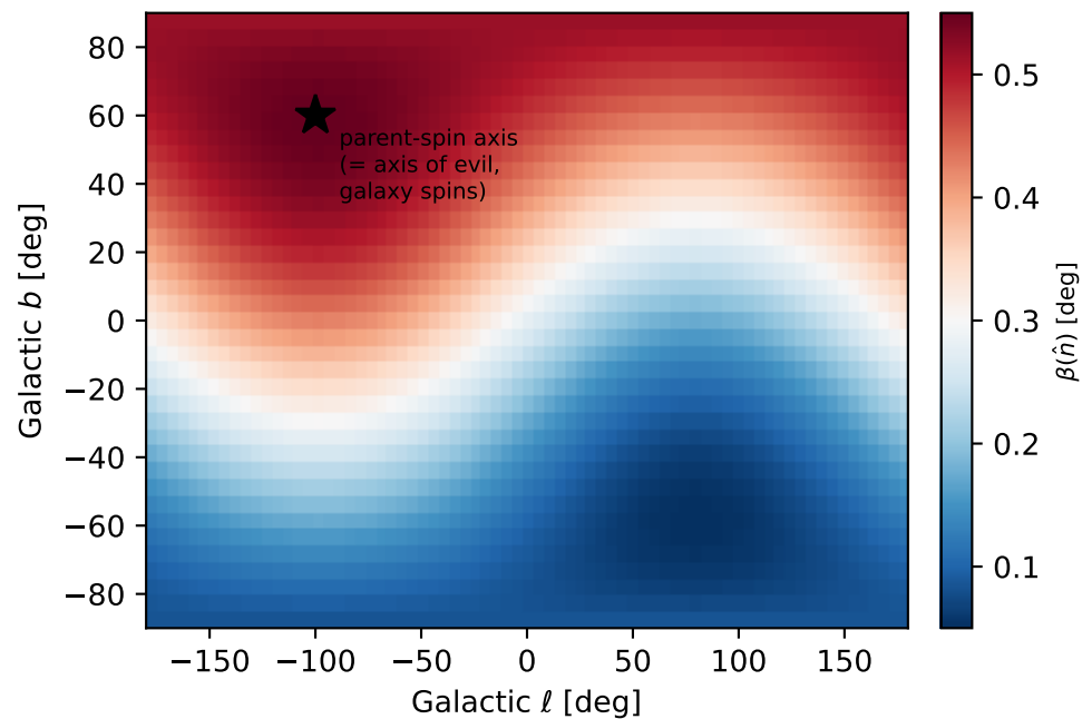
Distinctive: anisotropic \beta(\hat{n}) locked to the inherited axis (schematic)
