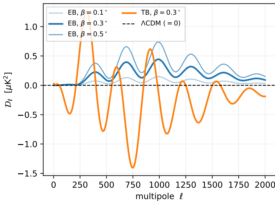
The parity-odd fingerprint (from real CAMB EE/TE)
