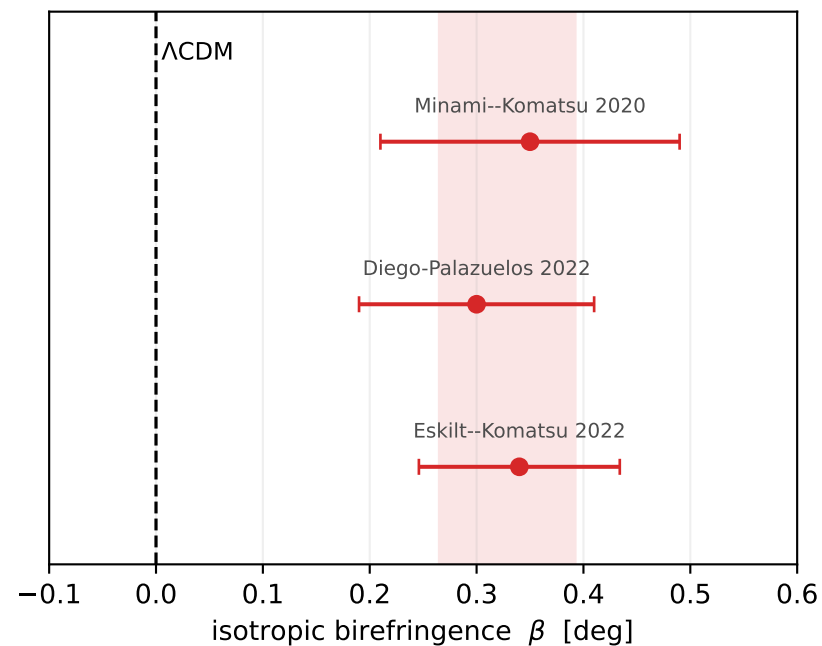
Measured: \beta \sim 0.3^\circ , \sim 3\sigma ( \Lambda CDM forbids it)
