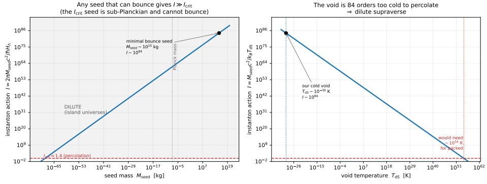
Figure 5.7: Computing the OG-nucleation instanton action, I = 2\pi M_{\text{seed}} c^2 / \hbar H_\Lambda (Equation (5.13)). Left: I versus seed mass; any seed massive enough to bounce ( M_{\text{seed}} \sim 10^{15} kg, the self-gravitating minimum) gives I \sim 10^{84} \gg I_{\text{crit}} \simeq 1.4 , the I_{\text{crit}} seed being sub-Planckian and unable to bounce. Right: I versus void temperature; the cold de Sitter void ( \sim 10^{-30} K) is eighty-four orders too cold to percolate. The verdict is robust: a dilute, eternal-inflation-like supravse of isolated island universes. Reproducible as figures/scripts/ch05_instanton.py.
