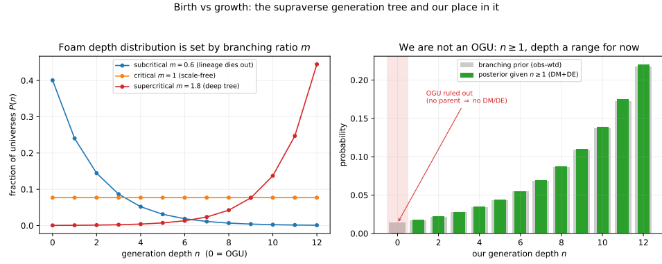
Figure 5.2: Where our universe sits in the generation tree. Left : the depth distribution (5.4) for sub-, near-, and super-critical branching m (the super-critical pile-up at the right edge reflects the hard truncation D used for illustration; a soft viability cutoff rounds it). Right : our posterior. The observation that we have dark matter and dark energy—both requiring a parent—zeroes the n = 0 (OGU) bin: we are not an original-generation universe. Generated by figures/scripts/ch05_population.py .
