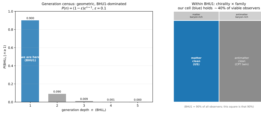
Figure 8.3: The supravverse census of viable observers. Left : the generation tower is geometric and BHU 1 -dominated; we are in the n = 1 bar. Right : within BHU 1 , the chirality × family breakdown—our cell (matter, clean; blue) holds ~40% of all viable observers, with an identical antimatter CPT twin. Our footprint is the typical, dominant cell.
