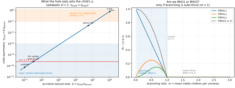
Figure 5.4: Left : the adiabatic bounce makes the child’s asymmetry equal to that of the accreted material, \eta_{\text{child}} = b \eta_{\text{parent}} (Equation (5.6)), splitting each lineage into a clean, photon-dominated family and a baryon-rich, degenerate one. Our \eta \simeq 6 \times 10^{-10} places our progenitor at a fair-sample accretor ( b \sim 1 ), not a star-fed one. Right : given n \geq 1 , P(\text{BHU}_n) \propto m^n ; we are likely \text{BHU}_{1-2} only if the branching ratio is subcritical ( m < 1 ), otherwise the population is deep. Reproducible as figures/scripts/ch05_accretion.py.
