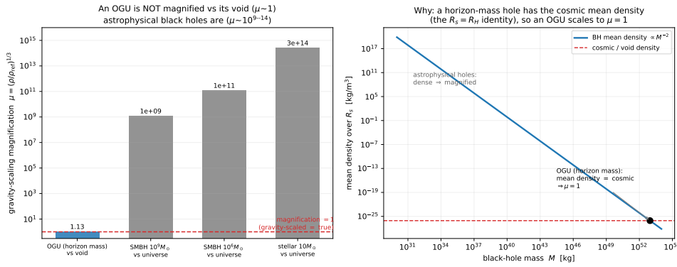
Figure 10.1: Gravity-scaling magnification \mu = (\rho/\rho_{\text{ref}})^{1/3} . Left : an OGU (horizon mass, mean density = cosmic) sits at \mu \simeq 1 —gravity-scaled coordinates equal true coordinates at the OGU/void level—while astrophysical black holes, far denser than their host universe, magnify by 10^9 – 10^{14} . Right : the black-hole mean density ( \propto M^{-2} ) crosses the cosmic/void line precisely at the horizon mass, which is why an OGU scales to unity (the R_s = R_H identity).
