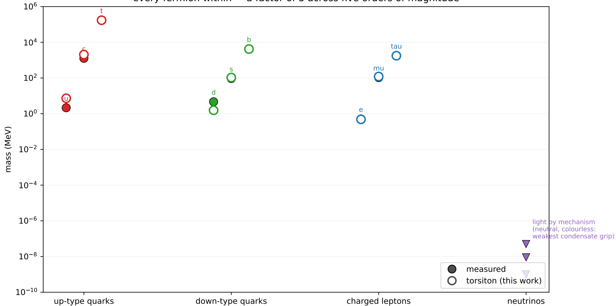
The torsiton mass spectrum vs experiment (physical units) every fermion within \sim a factor of 3 across five orders of magnitude
