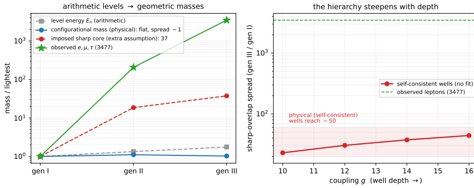
Figure 6.4: The generation overlap in the self-consistent well (derived couplings, no fitted shape), and why it is a conjecture not a result. Left : the three radial rungs have nearly even (arithmetic) level energies, but the physical configurational mass, Eq. (6.8), is flat —spread \sim 1 , no hierarchy—because the local mass M(r) is broad. A geometric spread appears only against an imposed sharp core (the dashed curve), which is an extra assumption beyond the configurational mass; where imposed, it does track the observed lepton shape (lightest generation anomalously light) but not its size (3477). Right : the imposed-substrate spread grows with the well depth, but the minimal self-consistent soliton binds only \sim 1 compact rung; a three-rung tower needs a far deeper/wider core than the mean field digs—the strong-dynamics question (the well depth) owed to the lattice. Reproducible as figures/scripts/appC_generations.py.
