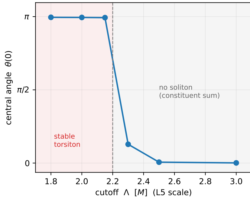
critical coupling \Lambda_c \approx 2.2 M
