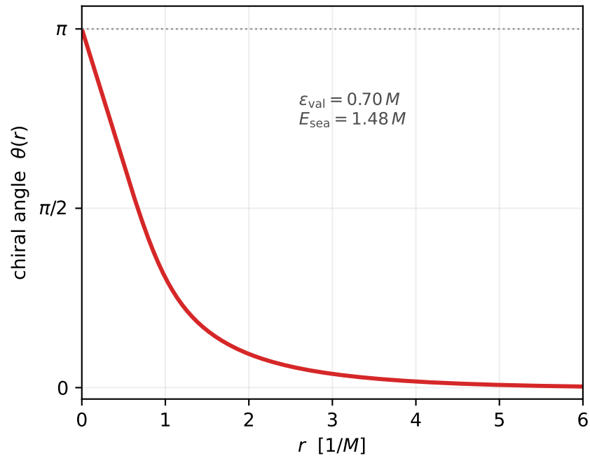
self-consistent torsiton ( \Lambda = 2M ): M \approx 3.6 M
