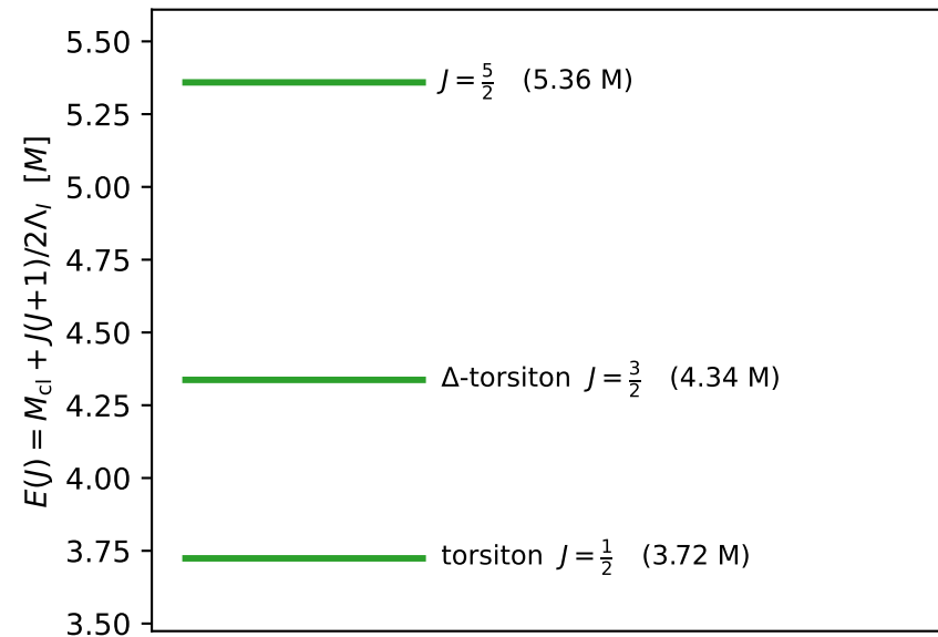
rotational band ( \Lambda_l = 2.4/M )
