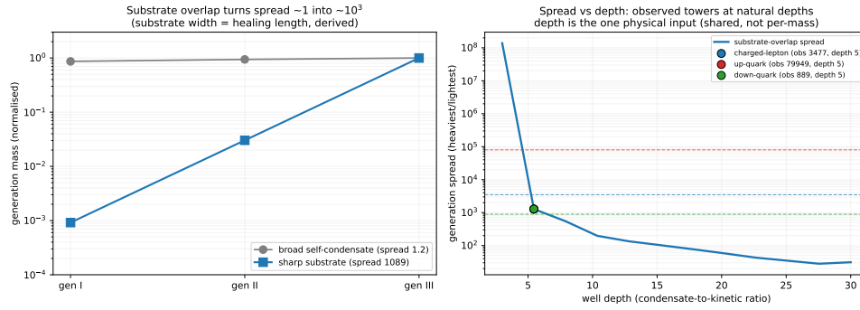
Figure 6.5: The substrate-overlap pass. Overlapping each generation with the sharply localized substrate (width = the well's healing length, derived) rather than the soliton's broad self-condensate turns the spread from \sim 1 into \sim 10^3 : the arithmetic level ladder of (6.5) becomes the observed geometric mass hierarchy, with no new fit.
