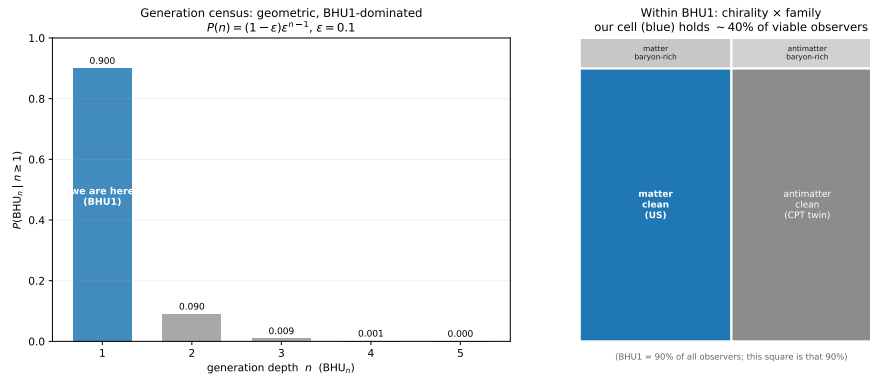
Figure 8.3: The supravarse census of viable observers. Left : the generation tower is geometric and \text{BHU}_1 -dominated; we are in the n = 1 bar. Right : within \text{BHU}_1 , the chirality \times family breakdown—our cell (matter, clean; blue) holds \sim 40\% of all viable observers, with an identical antimatter CPT twin. Our footprint is the typical, dominant cell.
