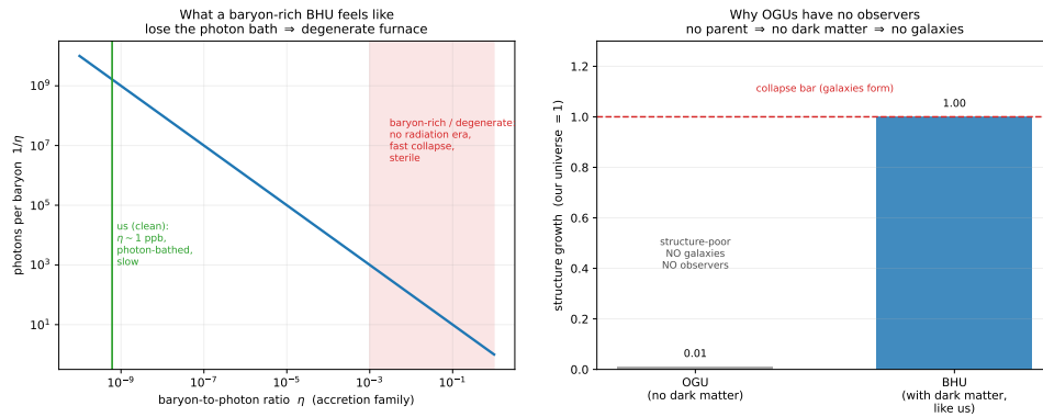
Figure 8.4: What other universe types are like. Left : along the accretion-family axis, photons per baryon 1/\eta —our clean cosmos ( \eta \sim 1 ppb) is photon-bathed and slow, while a baryon-rich one ( \eta \rightarrow 1 ) has no radiation era and collapses fast into a degenerate, sterile furnace. Right : structure growth normalised to our universe—an OGU, having no parent and so no dark matter, grows baryon-only and clears only \sim 1\% of the collapse bar, forming no galaxies. Observers live in clean-family BHU n only; the OGU root and the degenerate tail are empty by prediction.
