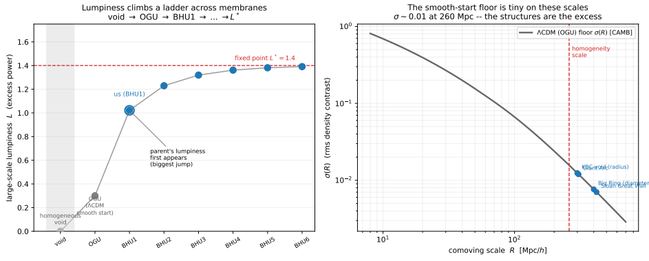
Figure 6.1: The lumpiness ladder. Left : large-scale lumpiness climbs from the homogeneous void through the OGU (minimal—the \Lambda CDM smooth-start case) to \text{BHU}_1 (us; the biggest jump, where the parent’s lumpiness first appears) and on toward a fixed point L^* . Right : the smooth-start floor \sigma(R) computed with CAMB falls from \sigma_8 \simeq 0.81 to \sim 0.01 by the 260 Mpc homogeneity scale, so the observed ultra-large structures (markers) sit far above what a singular start builds—they are the inherited rung, marking us as a BHU.
