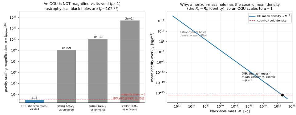
Figure 10.3: Gravity-scaling magnification \mu = (\rho/\rho_{\text{ref}})^{1/3} . Left : an OGU (horizon mass, mean density = cosmic) sits at \mu \simeq 1 —gravity-scaled coordinates equal true coordinates at the OGU/void level—while astrophysical black holes, far denser than their host universe, magnify by 10^9 – 10^{14} . Right : the black-hole mean density ( \propto M^{-2} ) crosses the cosmic/void line precisely at the horizon mass, which is why an OGU scales to unity (the R_s = R_H identity).
