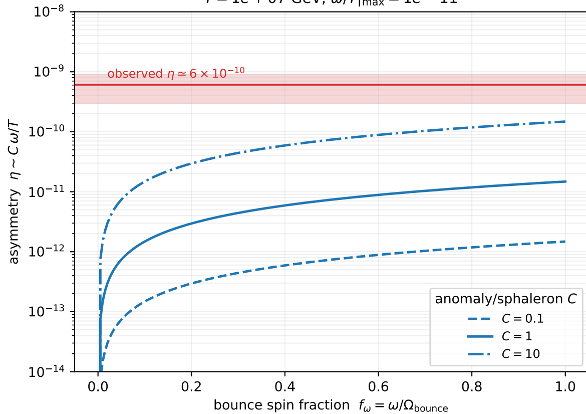
Track A: OGU manufactures \eta T \approx 1e+07 GeV, \omega/T|_{\max} \approx 1e-11
