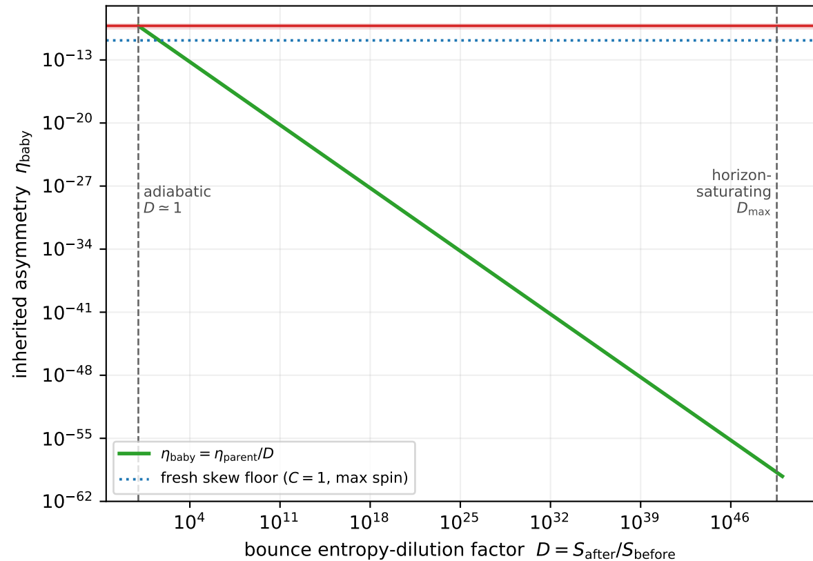
Track B: BHU inherits \eta observation selects the near-adiabatic end
