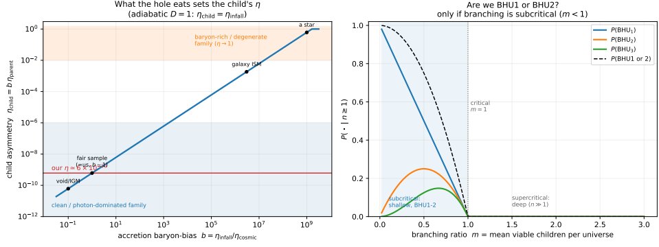
Figure 5.4: Left : the adiabatic bounce makes the child’s asymmetry equal to that of the accreted material, \eta_{\text{child}} = b \eta_{\text{parent}} (Equation (5.4)), splitting each lineage into a clean, photon-dominated family and a baryon-rich, degenerate one. Our \eta \simeq 6 \times 10^{-10} places our progenitor at a fair-sample accretor ( b \sim 1 ), not a star-fed one. Right : given n \geq 1 , P(\text{BHU}_n) \propto m^n ; we are likely BHU 1-2 only if the branching ratio is subcritical ( m < 1 ), otherwise the population is deep. Reproducible as figures/scripts/ch05_accretion.py.
