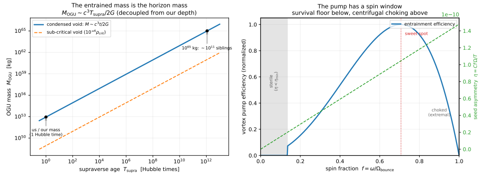
Figure 5.6: Left : the entrained OGU mass is the horizon mass of its causal patch, M_{\text{OGU}} \sim c^3 T_{\text{supra}} / 2G (Equation (5.10)): our mass at one Hubble time, \sim 10^{65} kg (and \sim 10^{11} siblings) at \sim 10^{12} Hubble times; a sub-critical void gives less. Right : the vortex pump has a spin window—a survival floor below (sterile) and centrifugal choking near extremal above—so genesis favours an intermediate spin sweet spot. The headline mass relation is robust; the efficiency shape is illustrative. Reproducible as figures/scripts/ch05_genesis.py .
