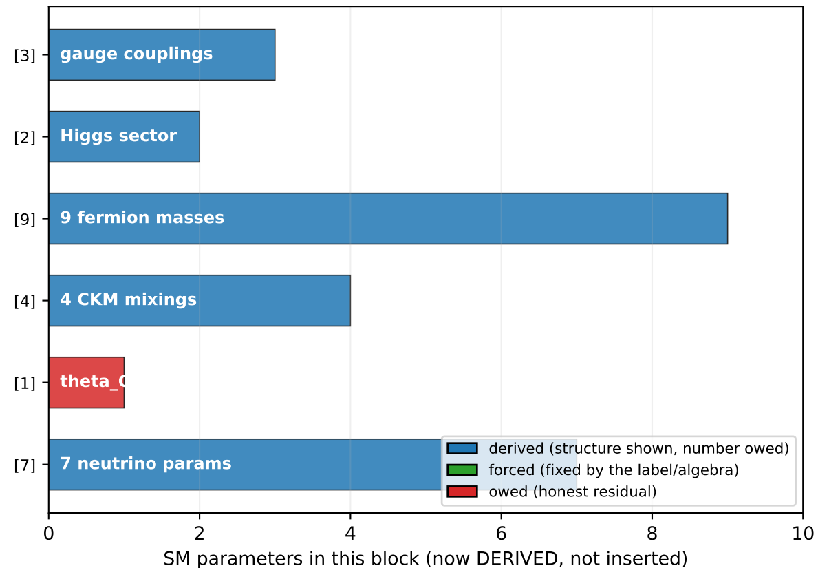
Eternal Dawn particle sector: 0 new fundamental parameters (all 26 traced to G, \hbar, c + generated \nu = f_\pi )
