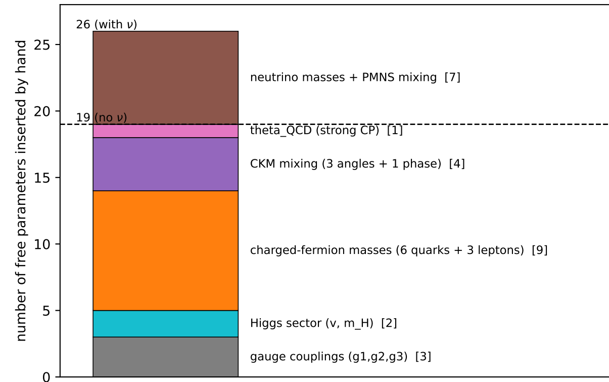
Standard Model: 19–26 free parameters (every block put in by hand)
